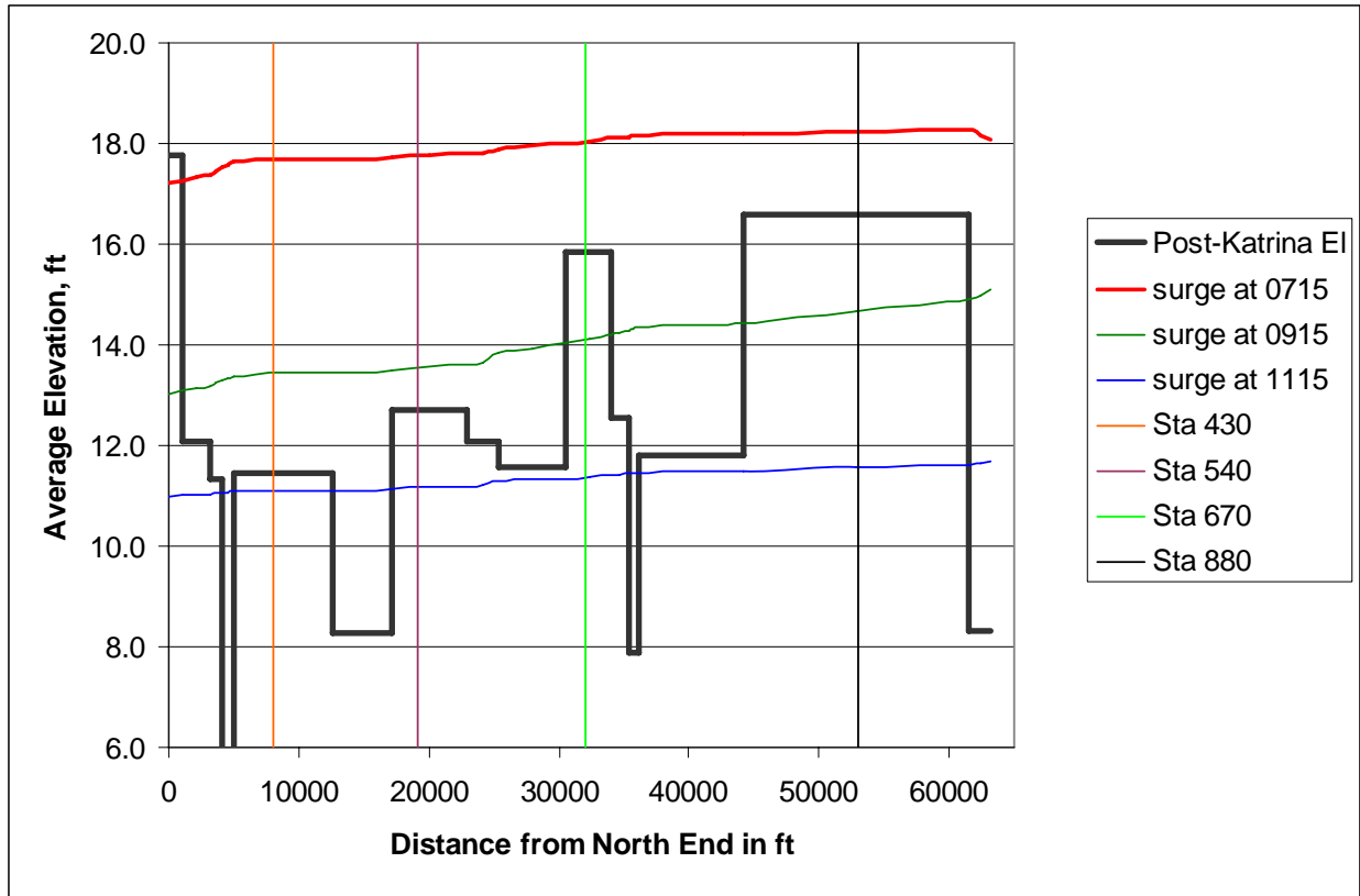
Figure 180. Post-Katrina average levee crest elevation, maximum surge level, post-peak surge levels, and Boussinesq analysis stations
