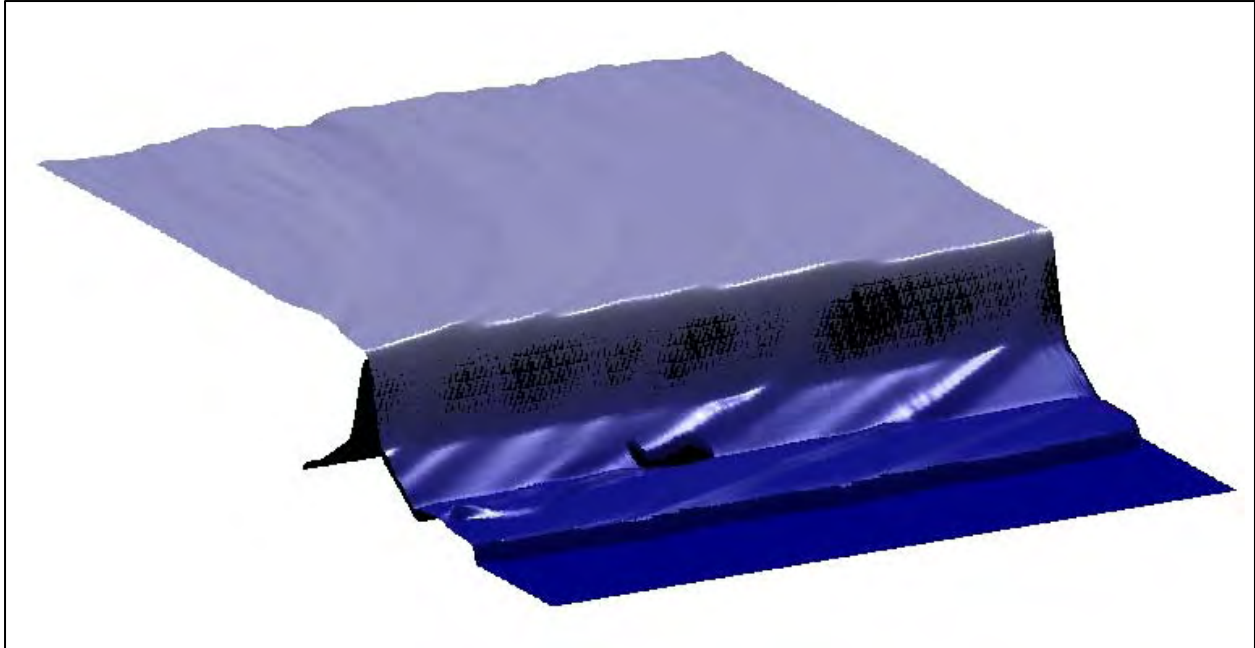
Figure 185. Side angle view of numerical waves overtopping the levee near the Paris Road Bridge. The levee is shown as the submerged black shape. View is looking towards the southwest; waves are from the east (left side of image)
