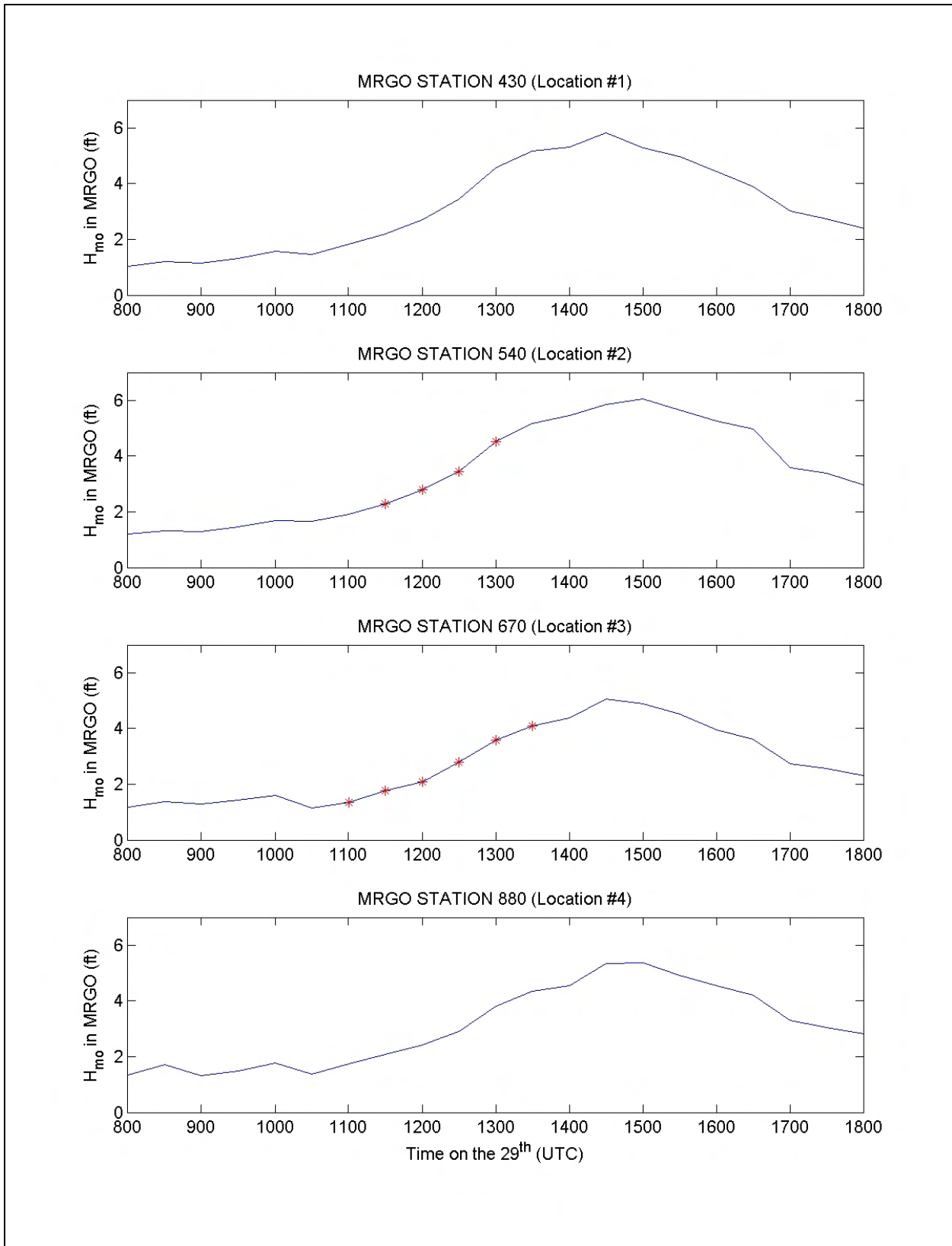
Figure 166. Time series of significant wave heights at the four locations shown in Figure 164
