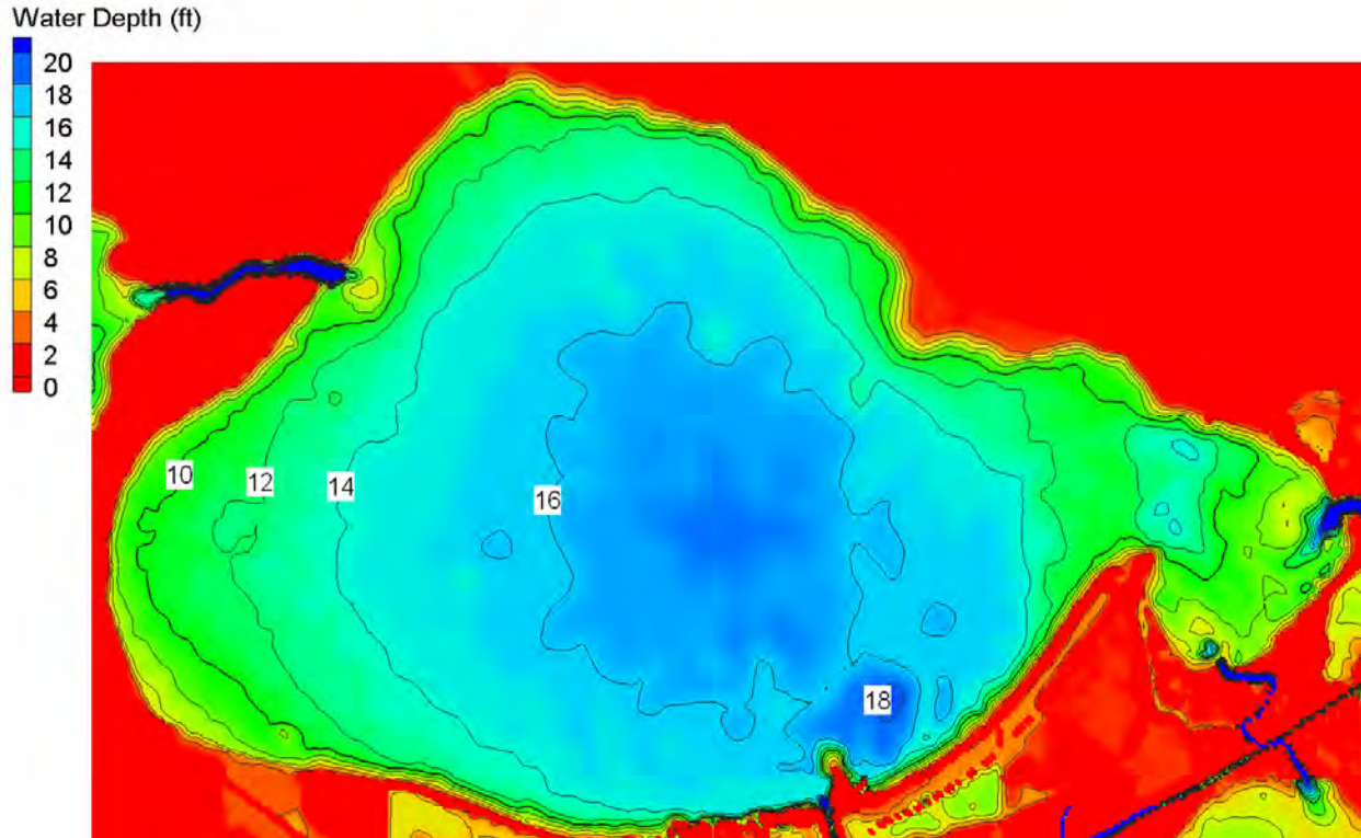
Figure 47. Lake Pontchartrain bathymetry grid (elevations in feet, NAVD88)
