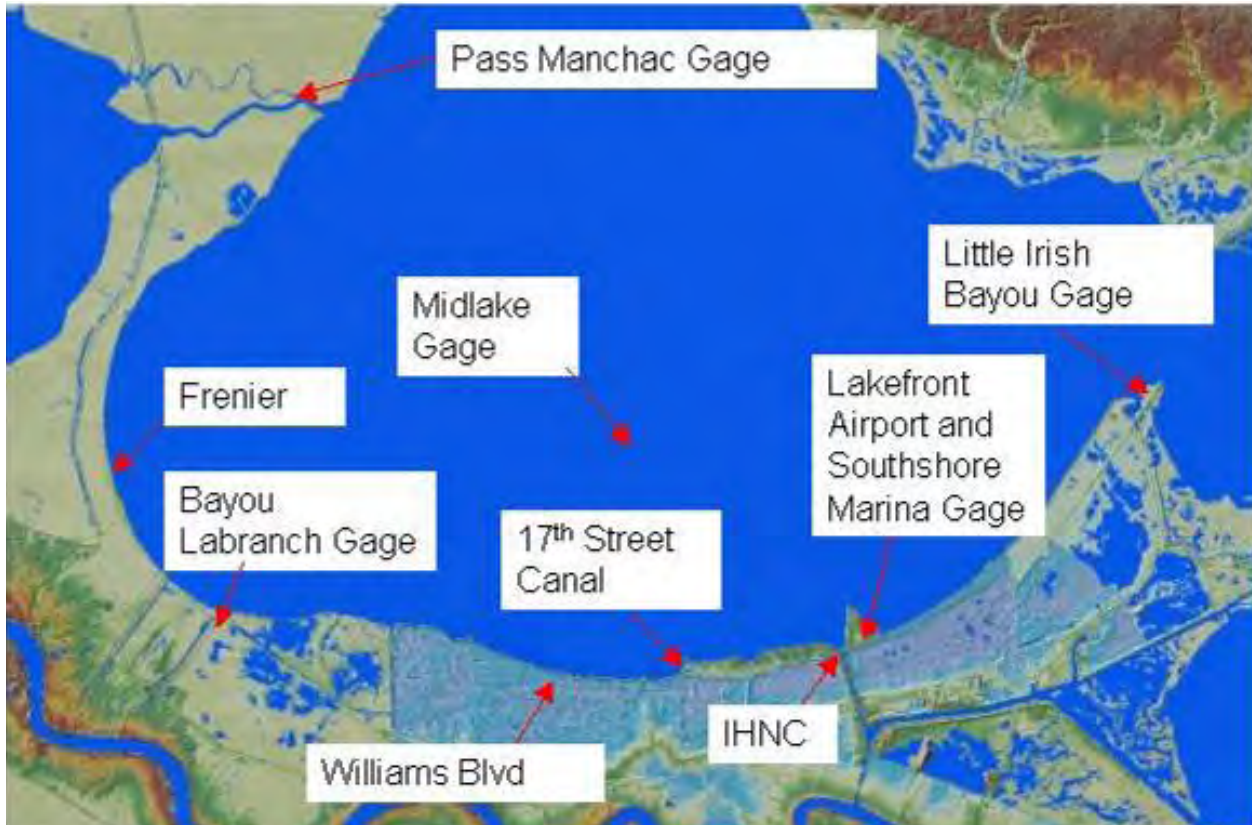
Figure 10. Lake Pontchartrain hydrograph locations
