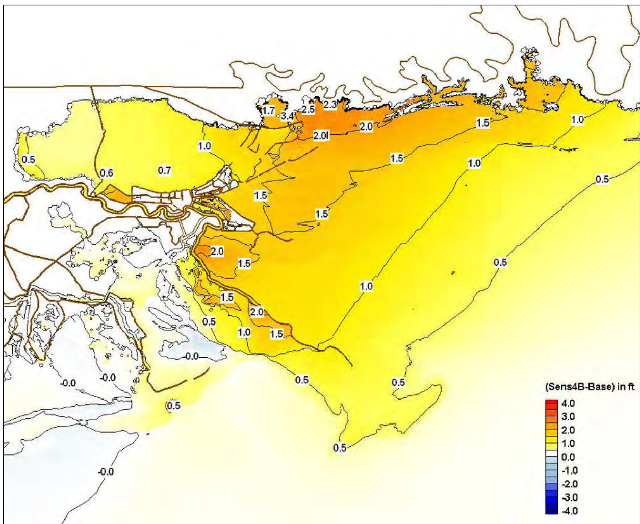
Figure 96. Difference in peak surge between sensitivity simulation with 5% increase in wind speed and the base simulation
