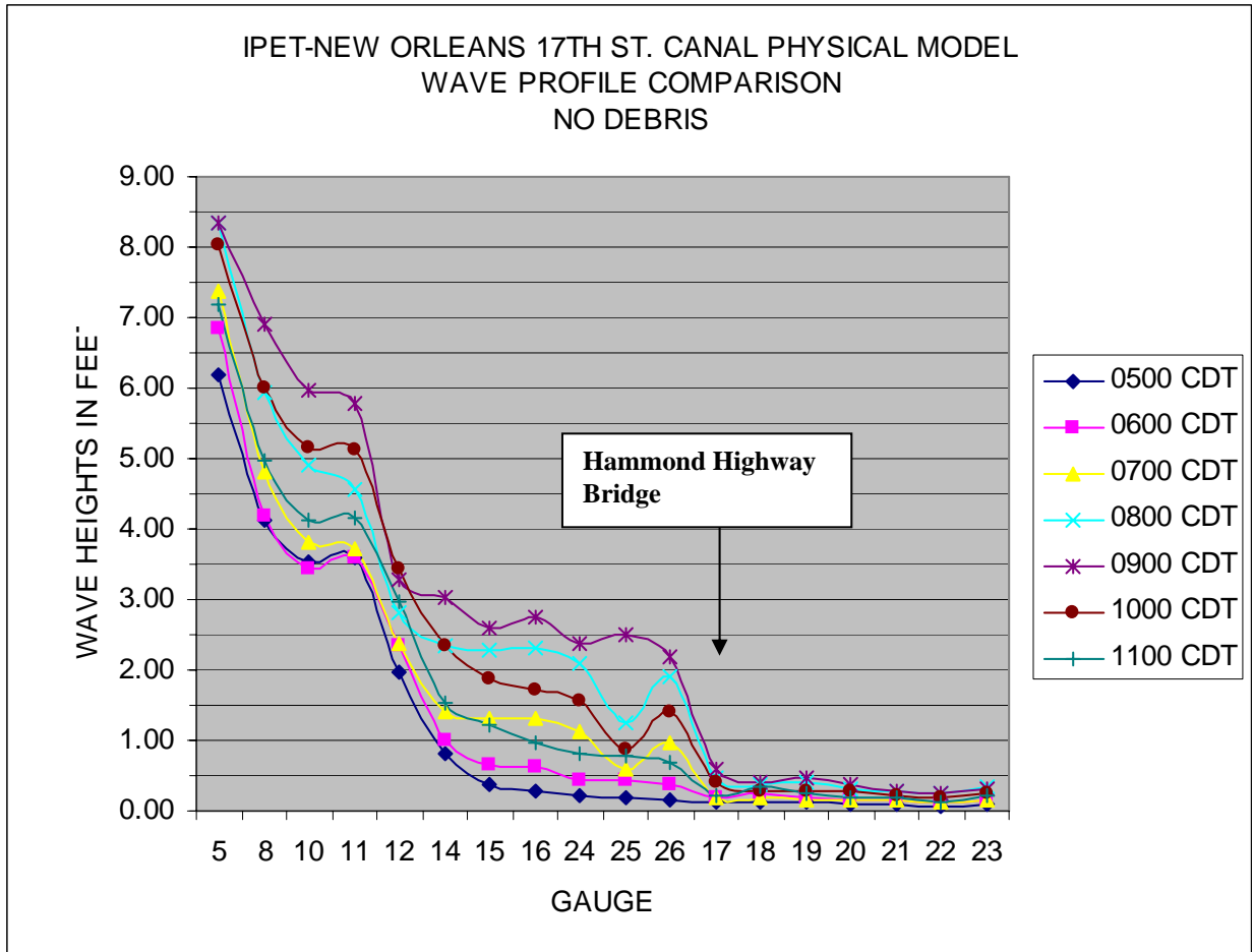
Figure 148. Decay of significant wave height at various times as the waves approach and enter the 17th Street Canal
