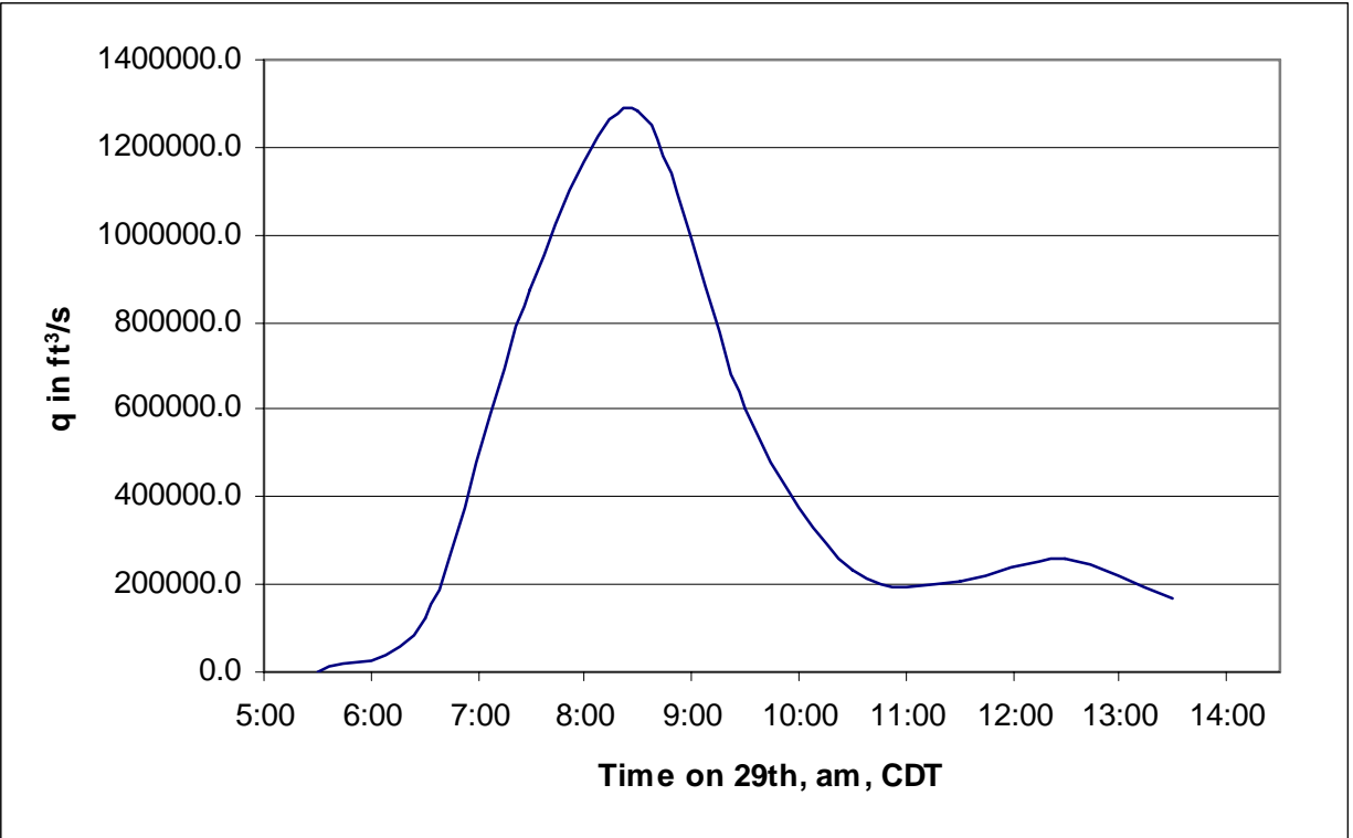
Figure 181. Integrated volumetric overtopping as a function of time for the MRGO levee for lower surge level
