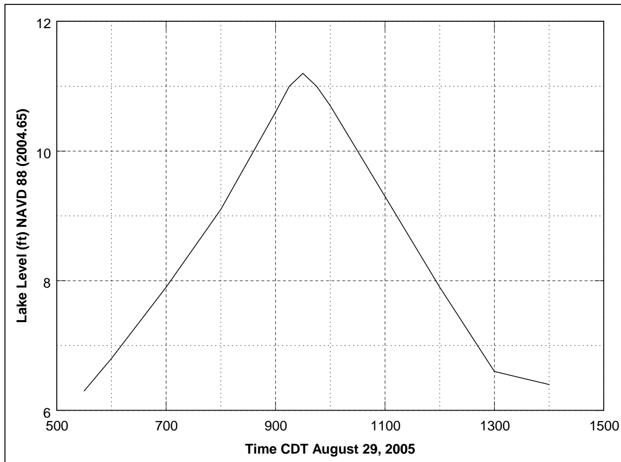
Figure 152. Reconstructed water levels in Lake Pontchartrain near north end of Orleans Canal
