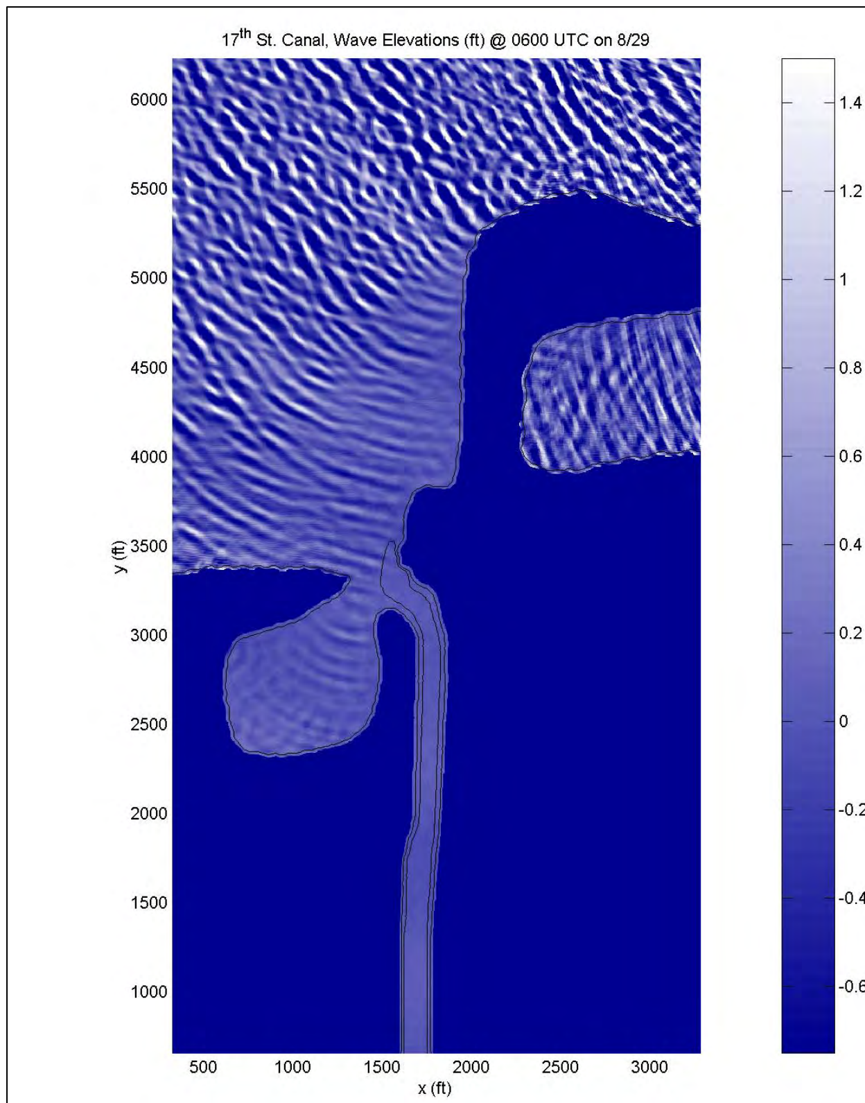
Figure 149. Snapshot of wave simulation at the 17th Street Canal entrance using the Boussinesq Model
