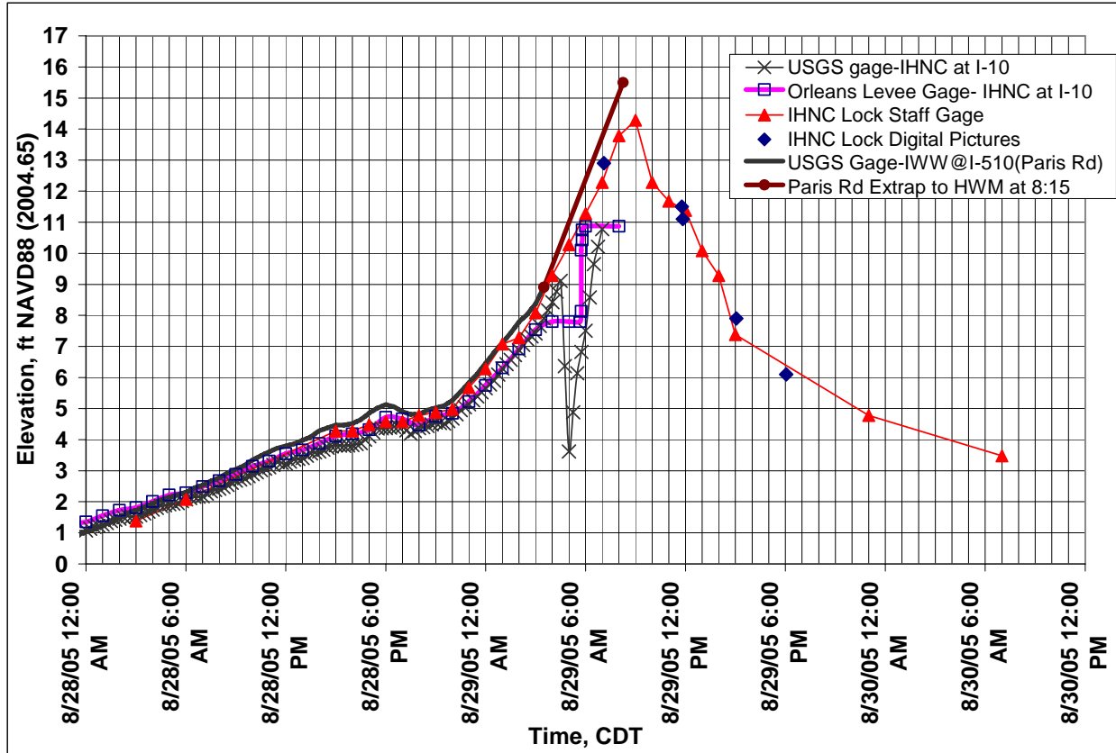
Figure 129. IHNC Hydrographs.
