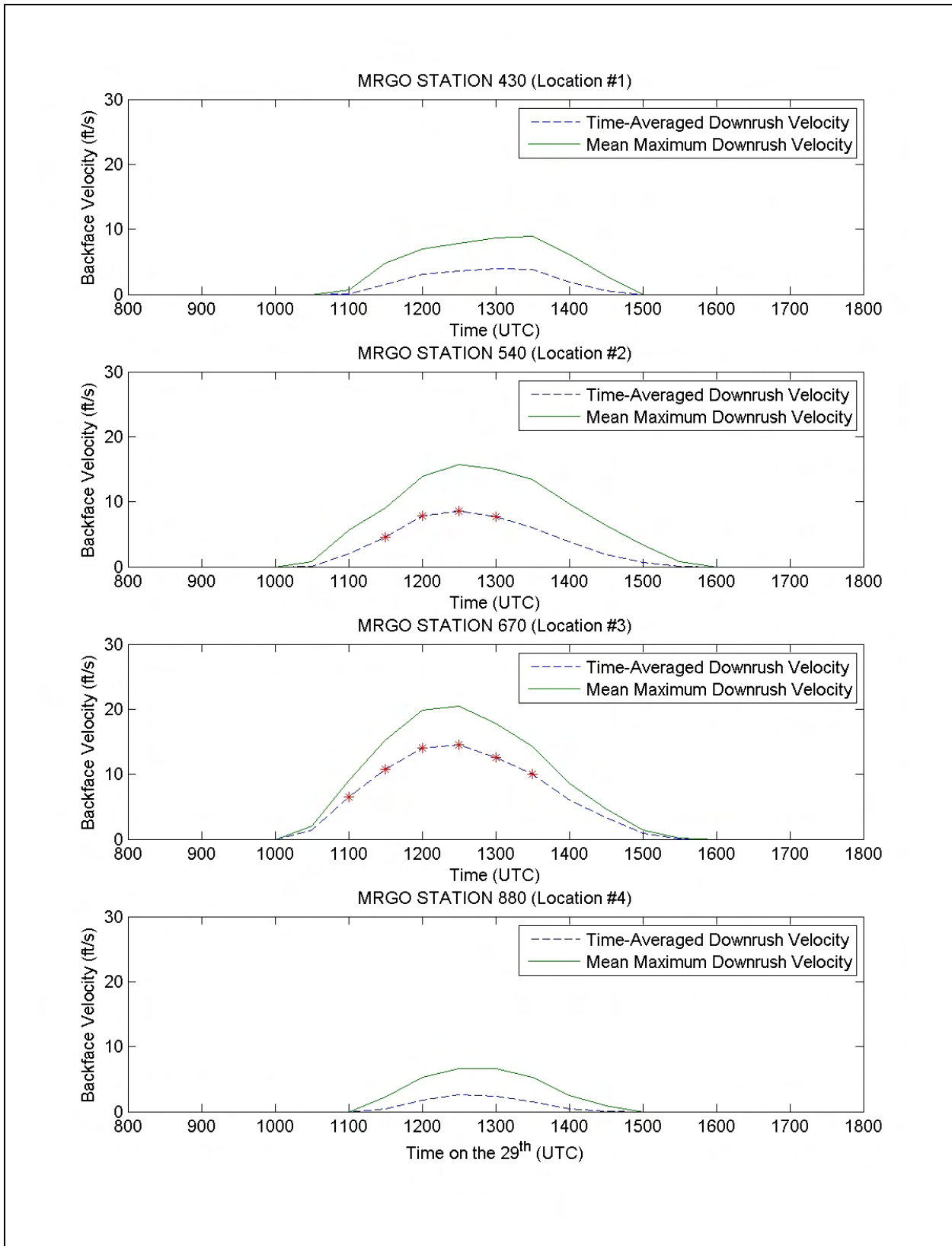
Figure 170. Velocities along the back face of the levees at the four locations shown in Figure 164
