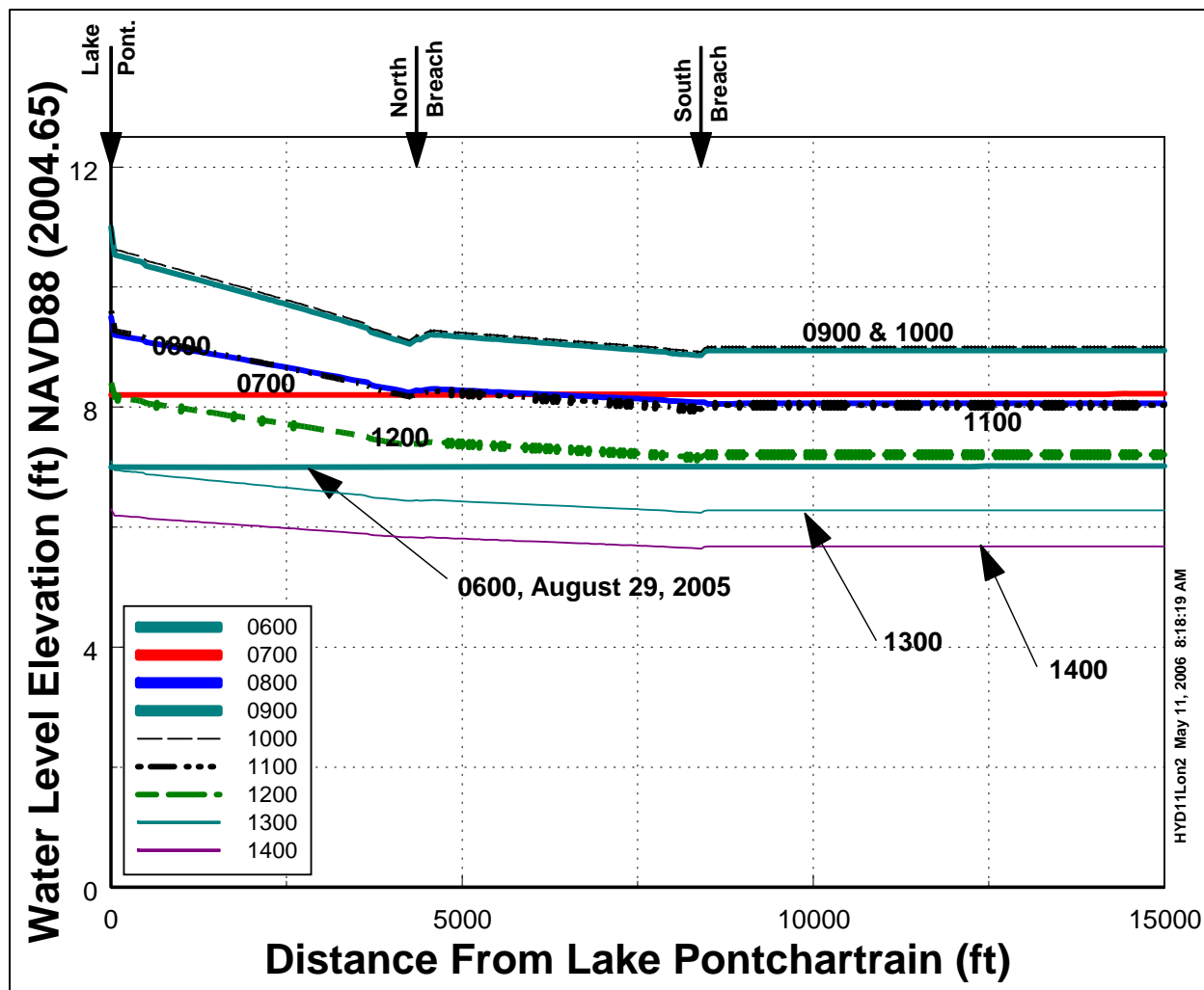
Figure 157. Water levels along London Avenue Canal for various times
