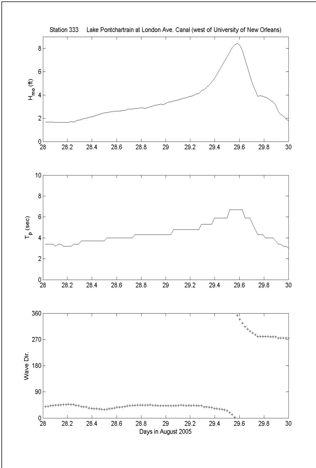
Figure 158. Time series of wave heights, periods and directions at the entrance to London Avenue Canal
