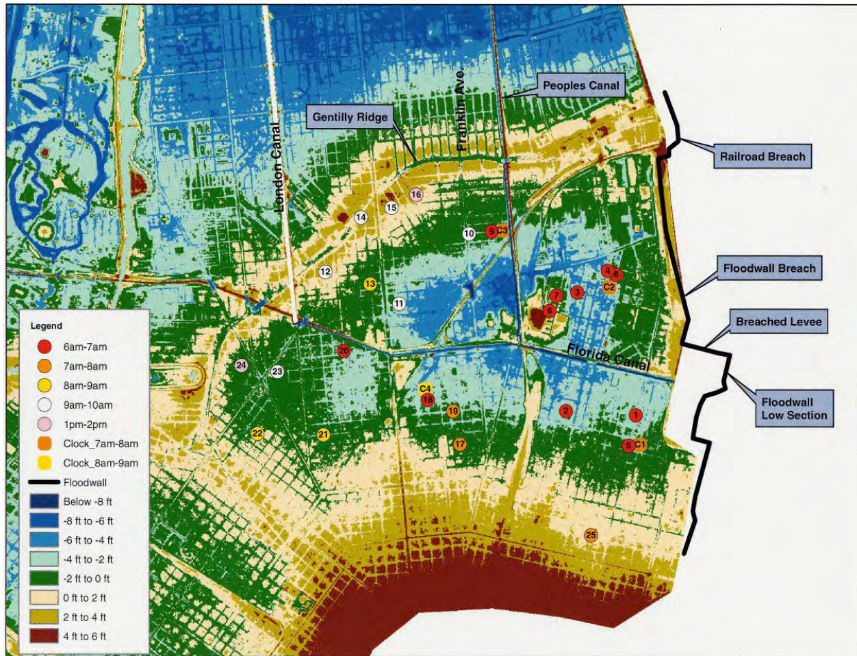
Figure 126. IHNC West area with approximate locations of eyewitness accounts and stopped clocks.
