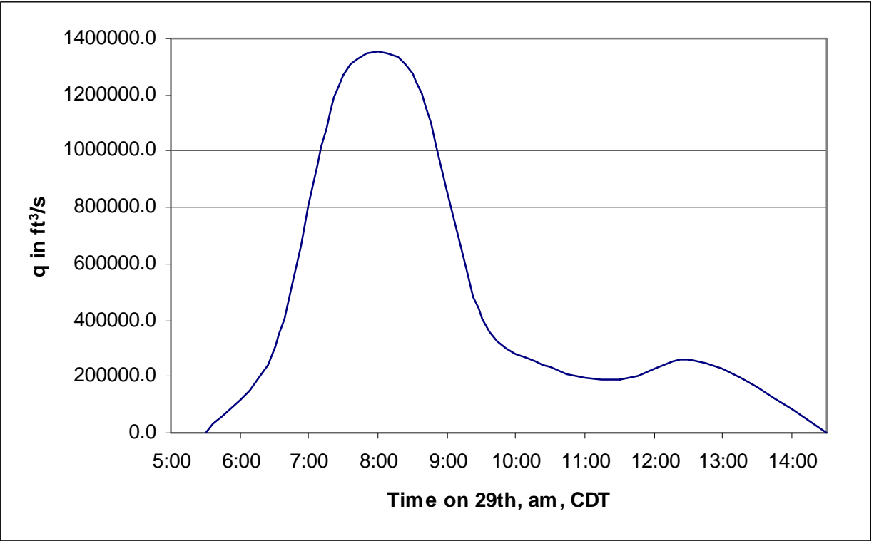
Figure 182. Integrated volumetric overtopping as a function of time for the MRGO levee for higher surge level
