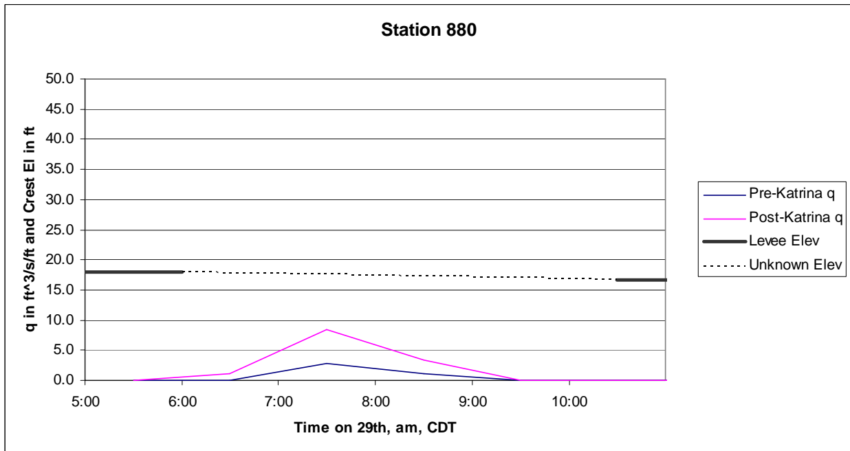
Figure 178. Approximate overtopping rate and levee crest height during storm as a function of time for Station 880 using Equation 1
