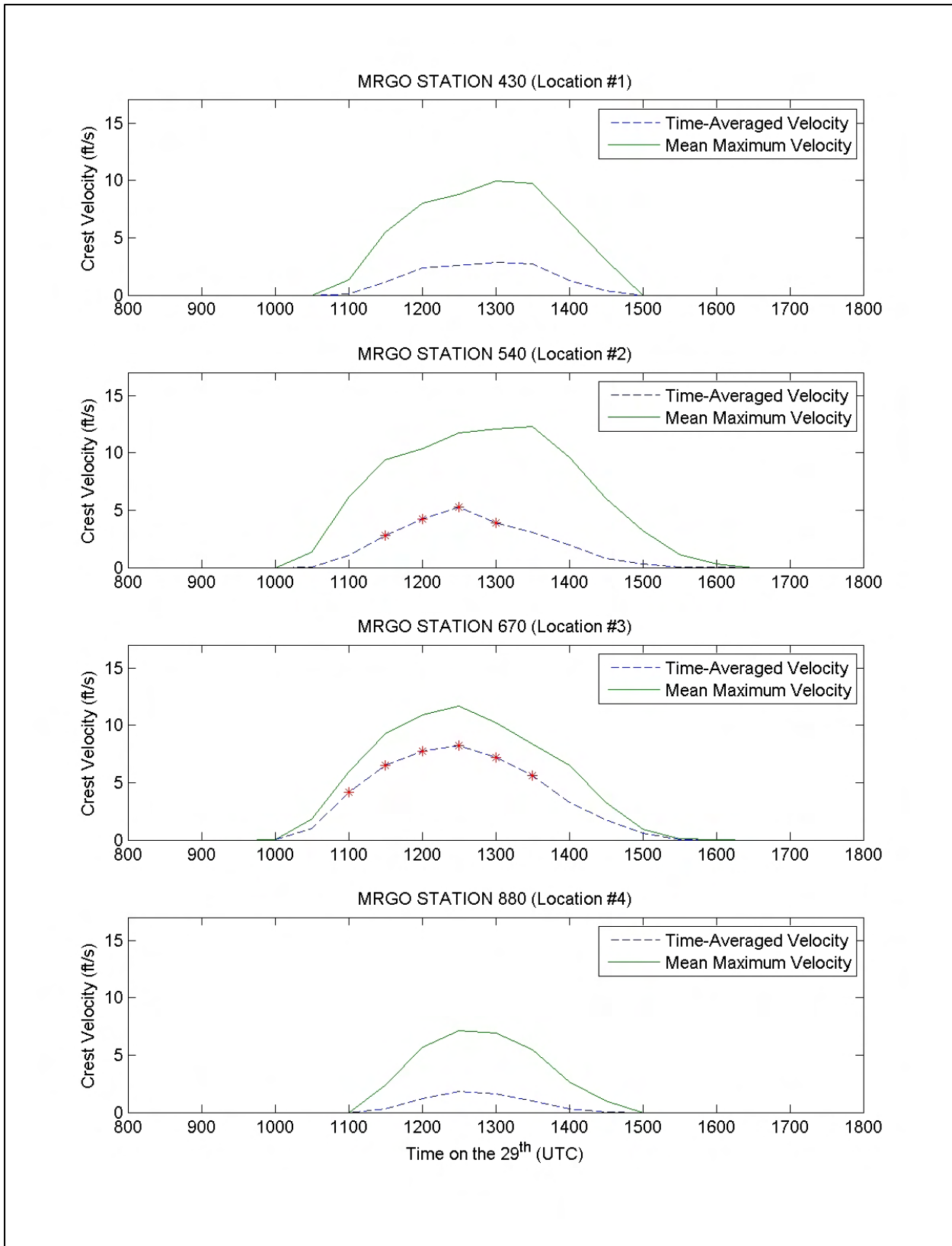
Figure 168. Estimated velocities over levee crest for the four locations shown in Figure 164
