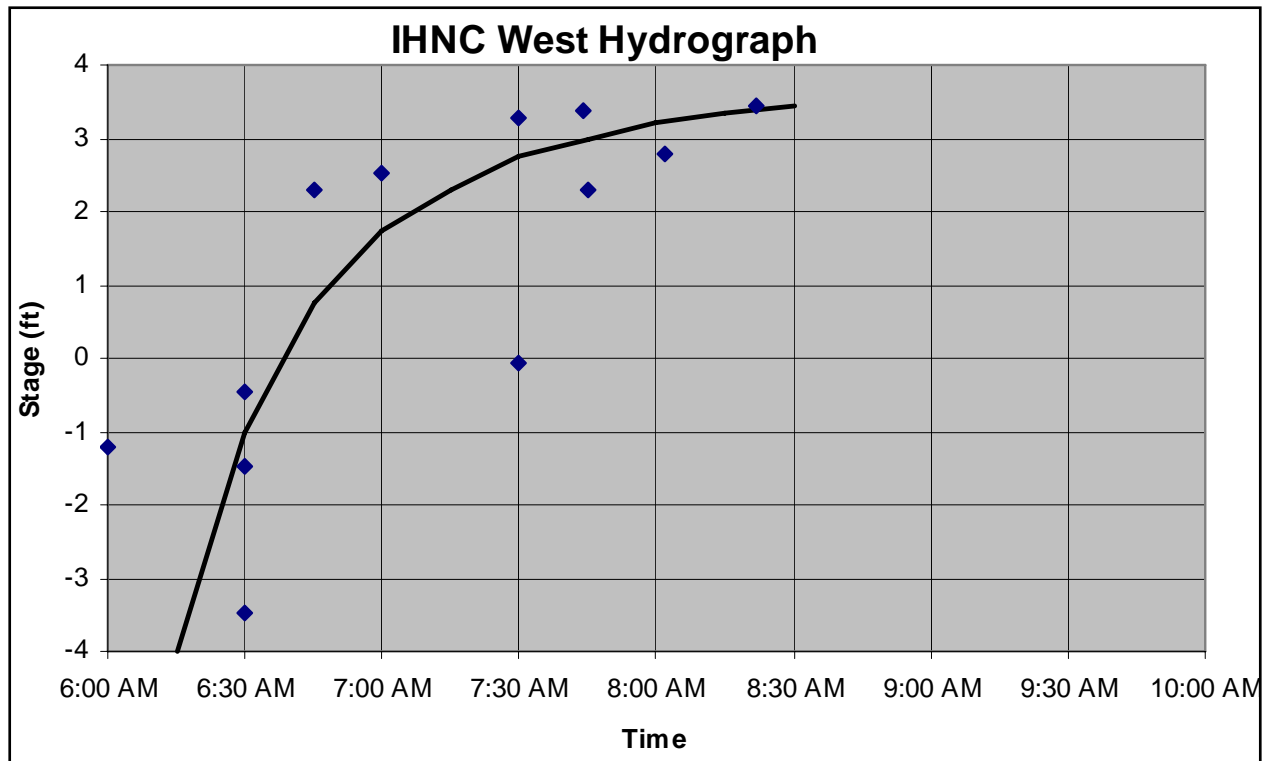
Figure 128. IHNC West hydrograph based on eyewitness accounts and stopped clocks
