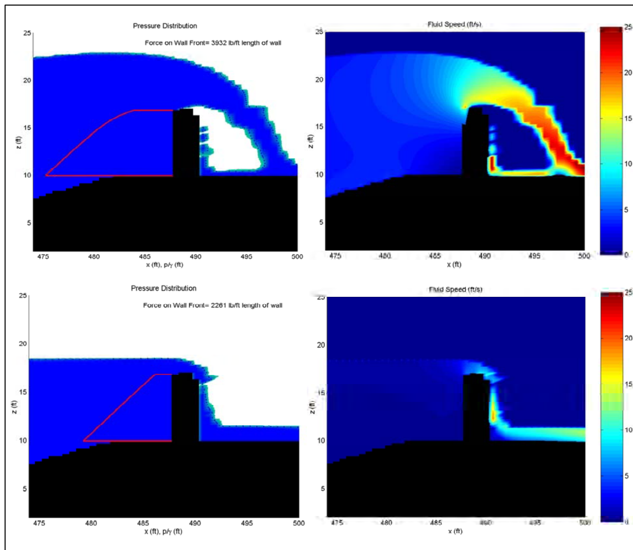
Figure 187. Pressure distribution (left) and speed field (right) under the wave crest (top) and wave trough (bottom) for wave overtopping the levee wall
