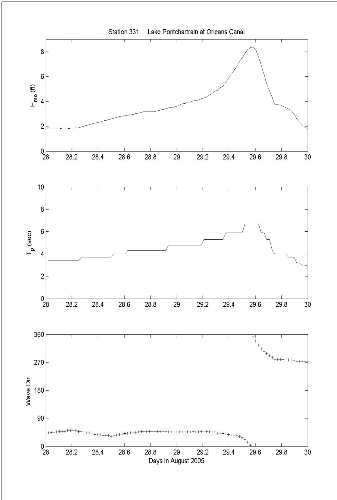
Figure 153. Significant wave height, wave period and wave direction in Lake Pontchartrain near north end of Orleans Canal
