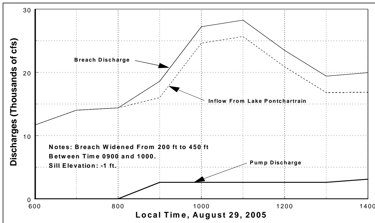
Figure 151. Time histories of breach and other discharges. Scenario 1
