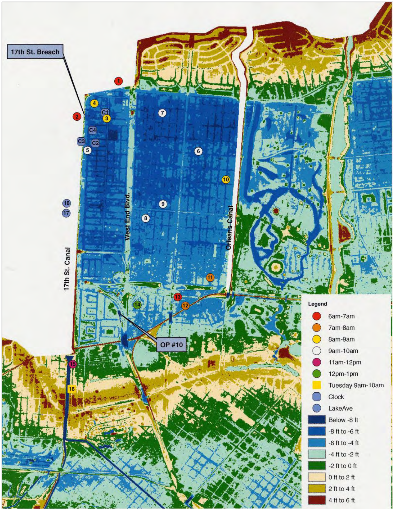
Figure 116. 17th Street area with approximate locations of eyewitness accounts and stopped clocks
