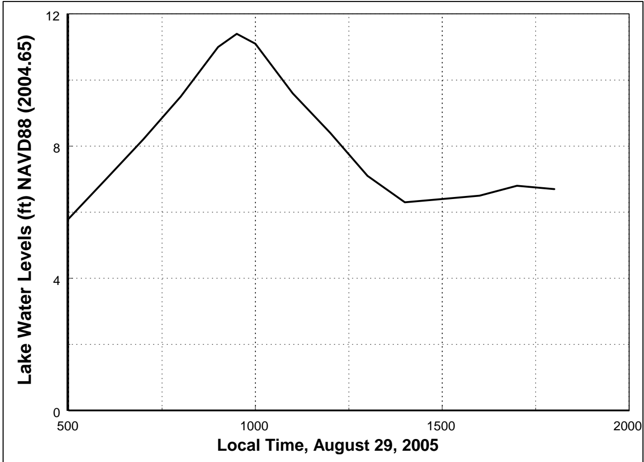
Figure 155. Estimated water levels in Lake Pontchartrain near north end of London Avenue Canal
