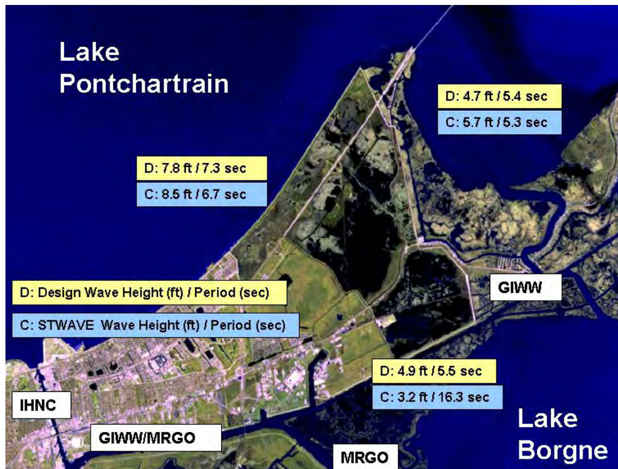
Figure 85. Wave maxima along eastern Orleans Parish hurricane protection system
