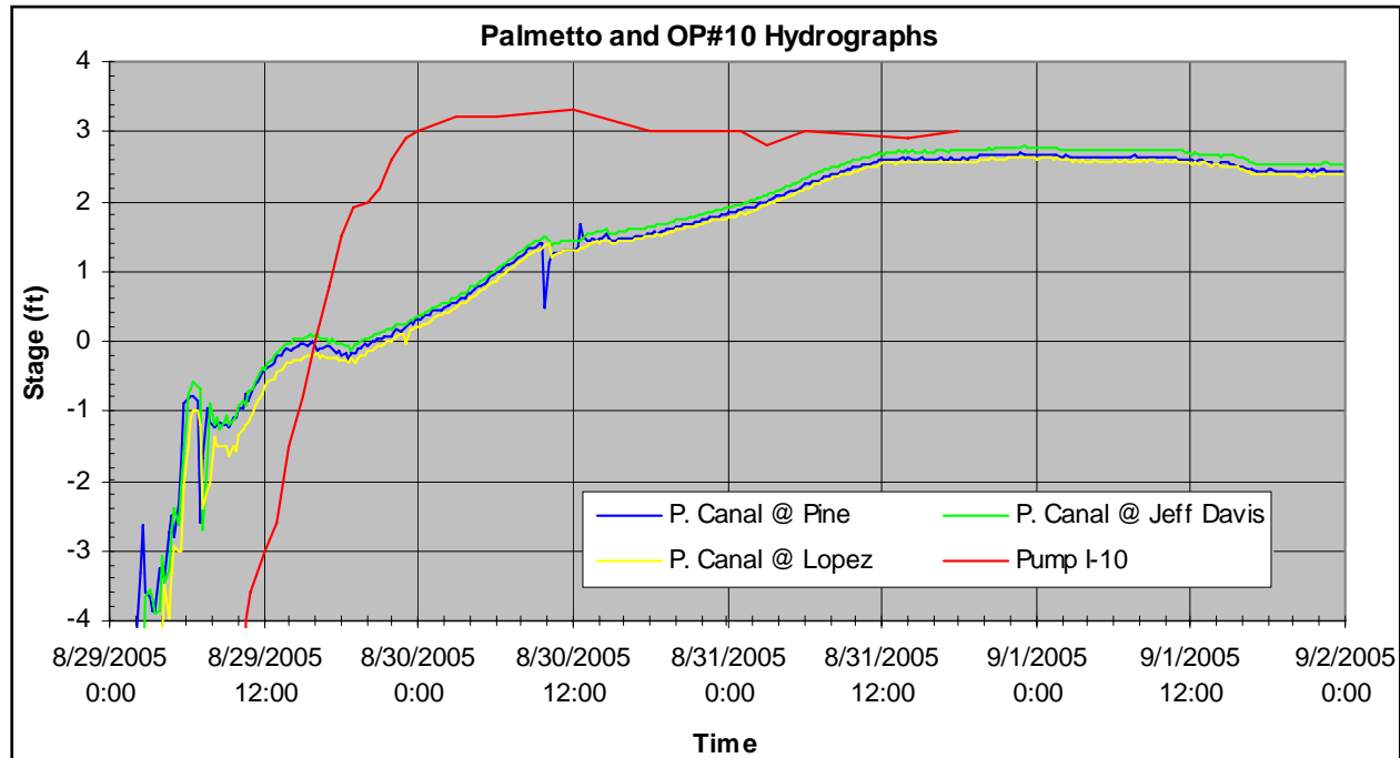
Figure 139. Stage hydrographs at Pump Station 10 and Palmetto Canal at Pine St., Lopez St., and Jeff Davis St.
