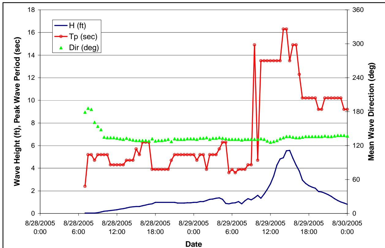
Figure 60. Temporal variation of significant wave height, peak period, and mean wave direction along the MRGO at Bayou Bienvenue
