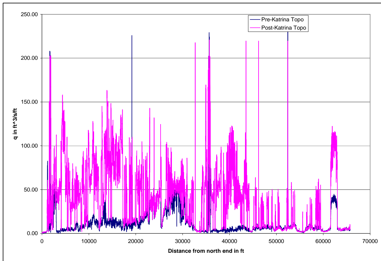
Figure 174. Overtopping rates for pre-Katrina and post-Katrina lidar survey crest heights along center line of MRGO levee corresponding to maximum surge elevation at approximately 0730 on the 29th
