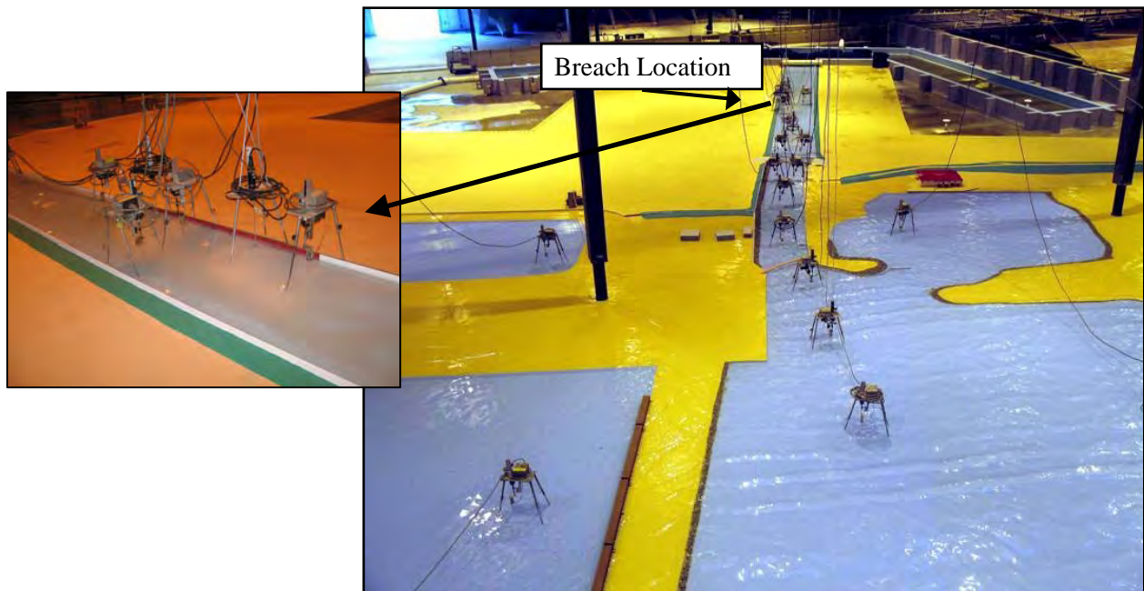
Figure 145. Views of 17th Street Canal model
