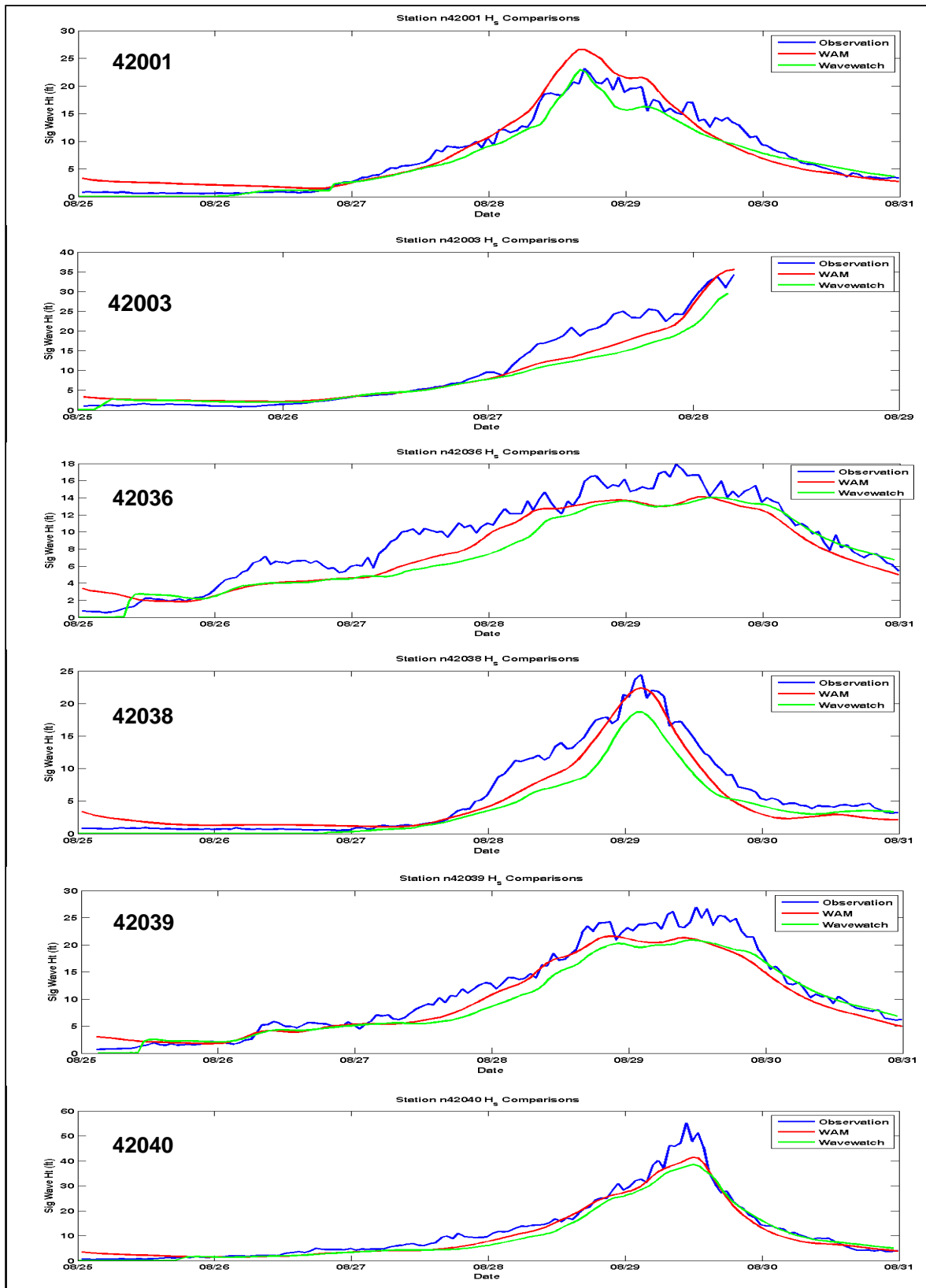
Figure 44. Comparison of significant wave heights (ft) as a function of time from observation stations (blue), WAM hindcast (red), and WAVEWATCH III hindcast (green).
