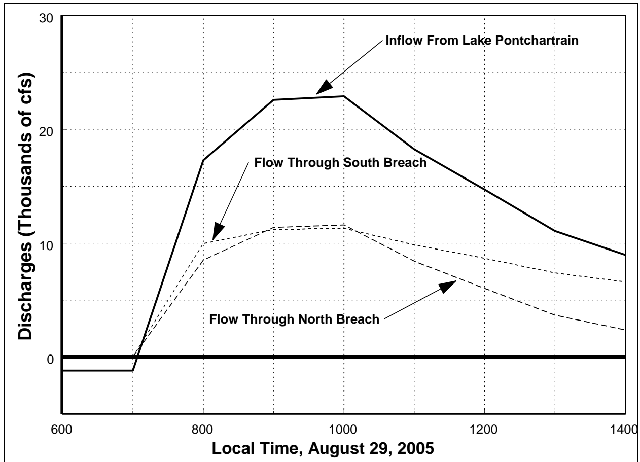
Figure 156. Time history of breach and lake discharges
