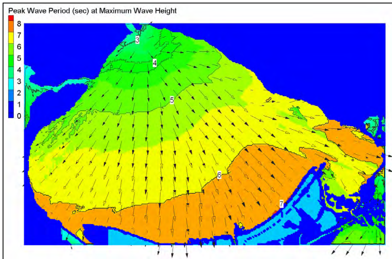
Figure 53. Lake Pontchartrain modeled peak wave period corresponding to the maximum significant wave height (periods in sec)
