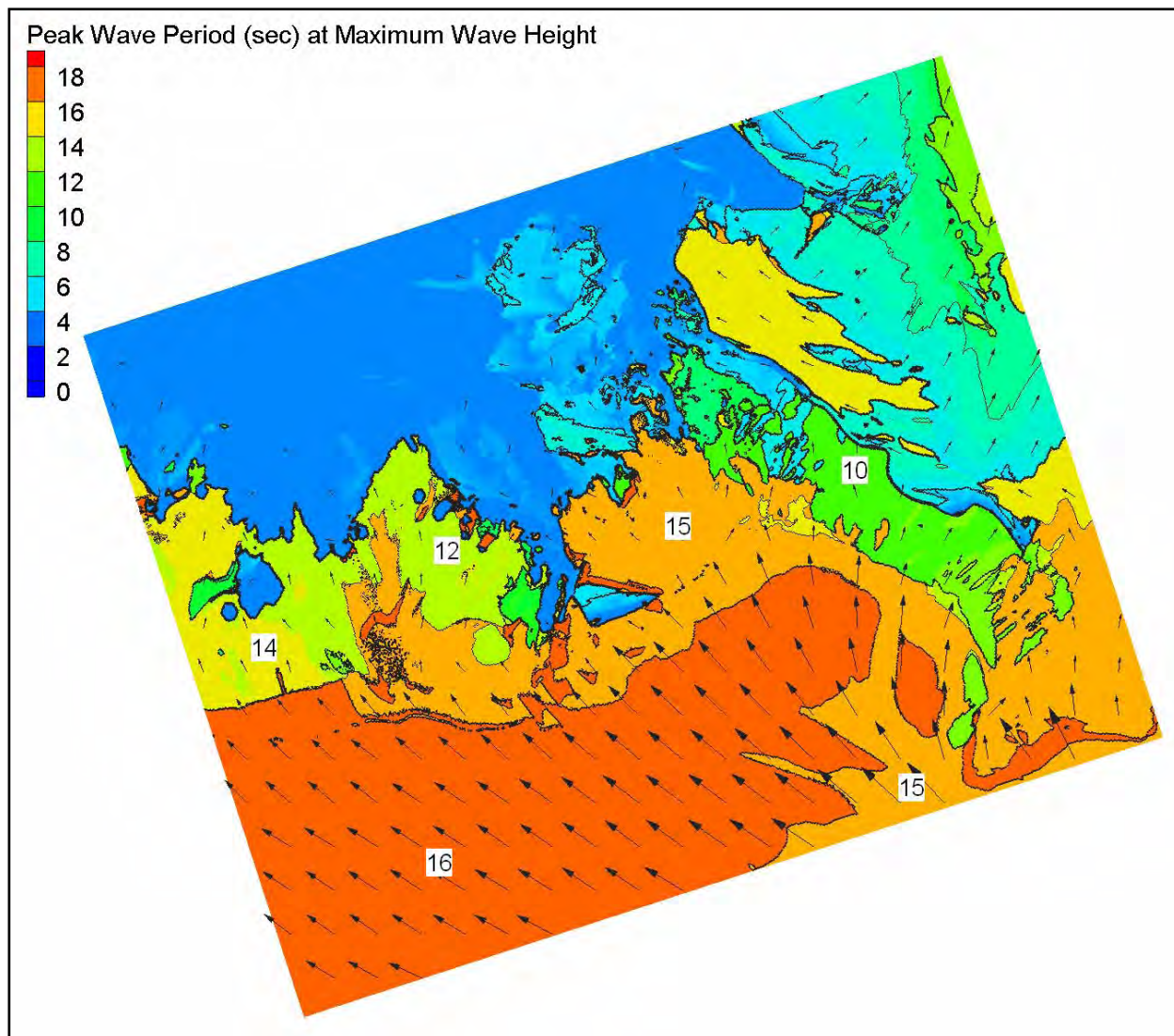
Figure 64. South Louisiana modeled peak wave period corresponding to the maximum significant wave height (periods in sec)
