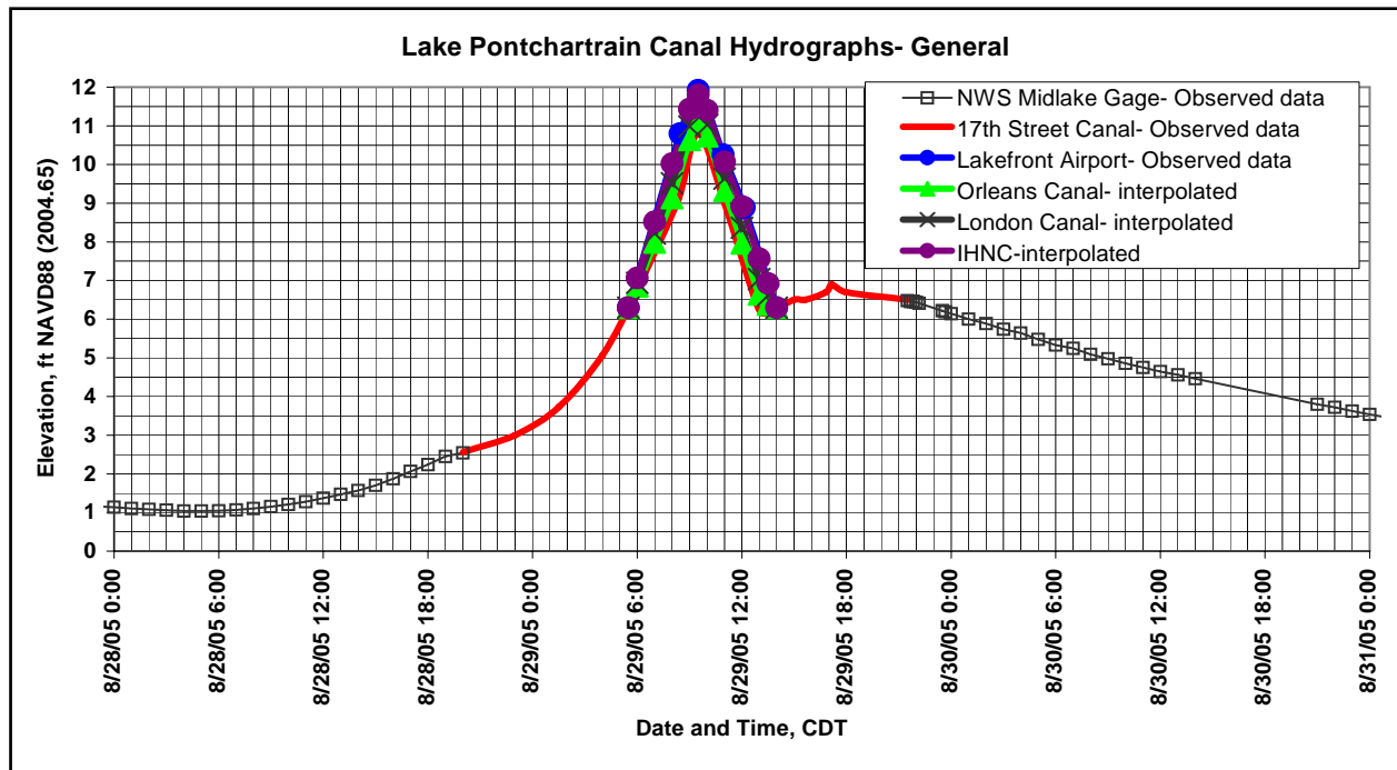
Figure 13. Constructed and interpolated hydrographs at canal entrances
