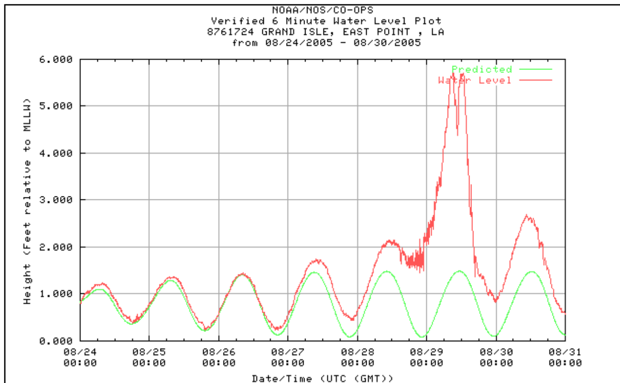
Figure 23. Hydrograph for NOAA National Ocean Service station at Grand Isle, Louisiana
