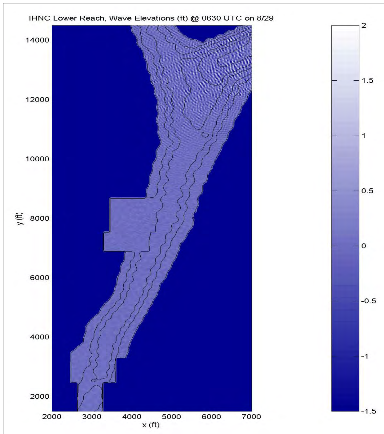
Figure 163. Region of IHNC modeled in Boussinesq simulations
