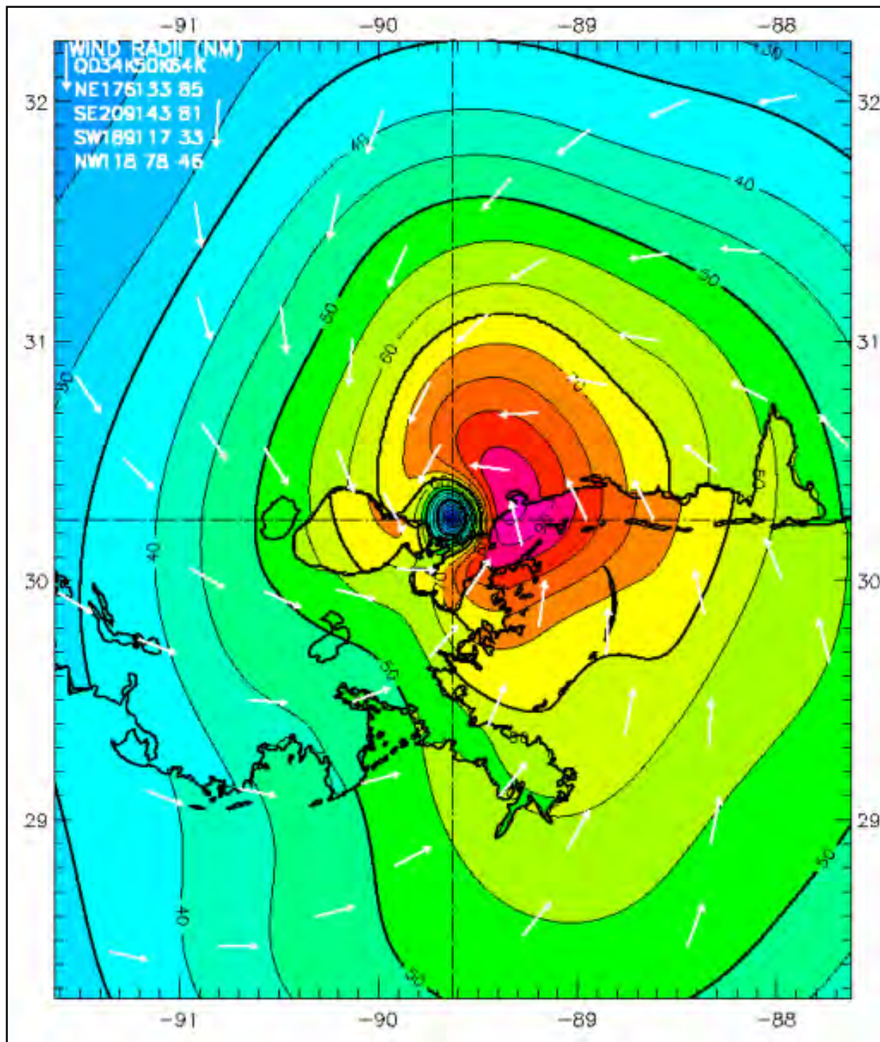
Figure 27. H*Wind snapshot for 1500 UTC on August 29, near landfall at MS/LA border
