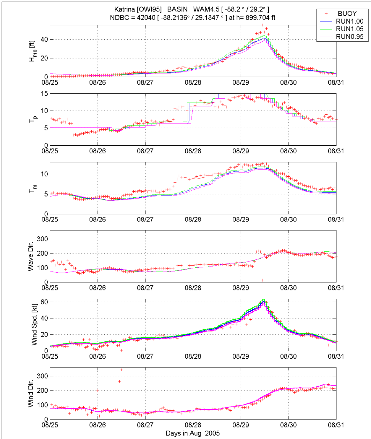
Figure 95. Comparison of WAM Cycle 4.5 basin-scale (blue line), sensitivity tests for plus 5 percent winds (green line) and minus 5 percent winds (magenta line) to the measurements at NDBC 42040.
