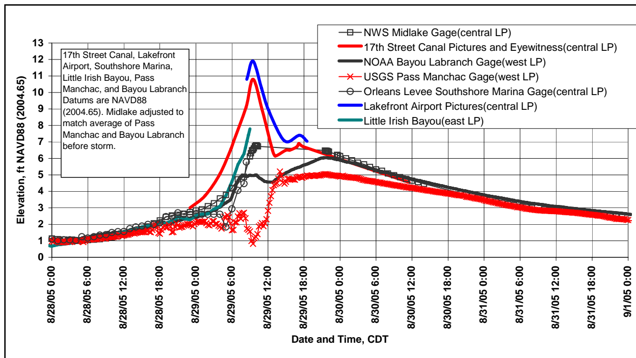
Figure 11. Gauge Hydrographs and Constructed Hydrographs on Lake Pontchartrain
