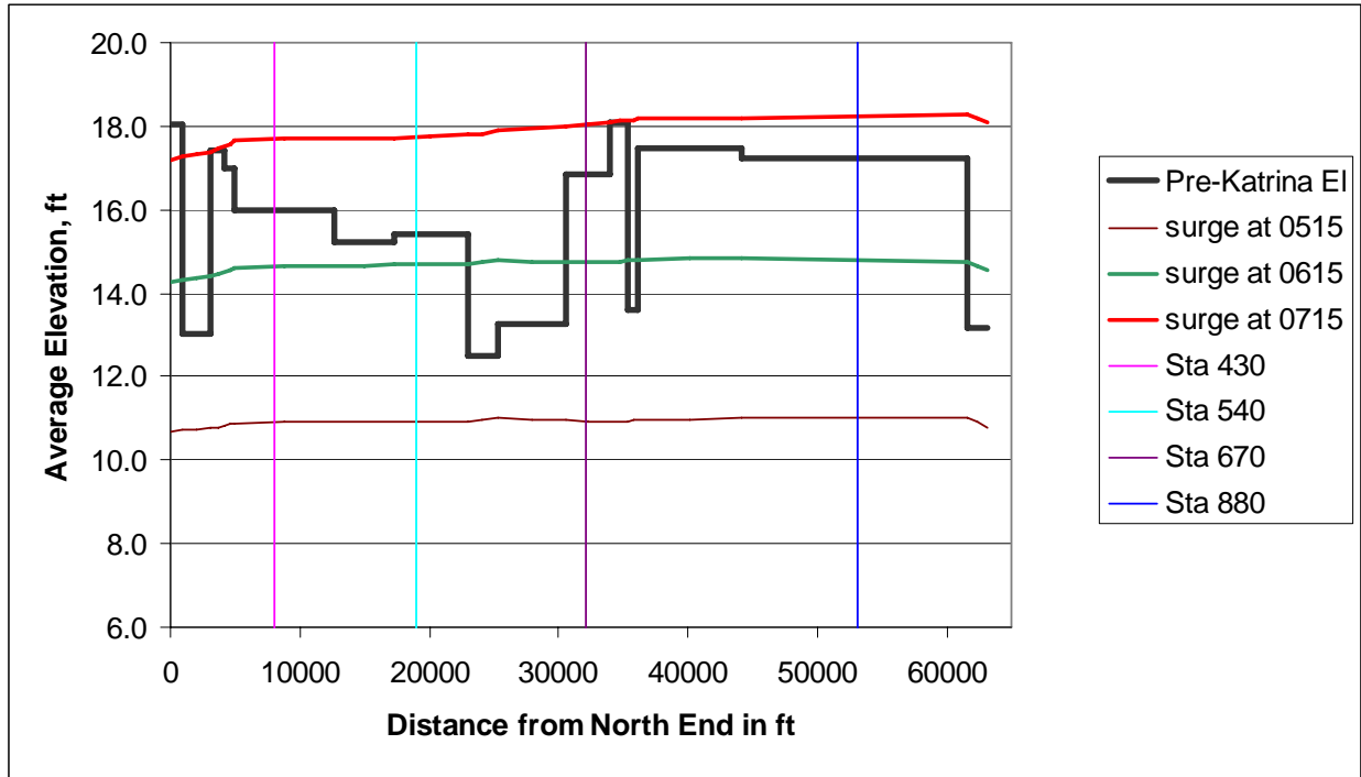
Figure 179. Pre-Katrina average levee crest elevation, pre-peak surge levels, maximum surge level and Boussinesq analysis stations
