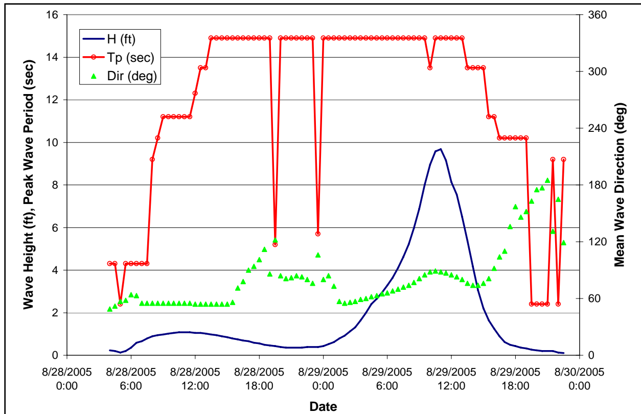
Figure 61. Temporal variation of significant wave height, peak period, and mean wave direction along the east-facing levee near Tropical Bend in south Plaquemines Parish
