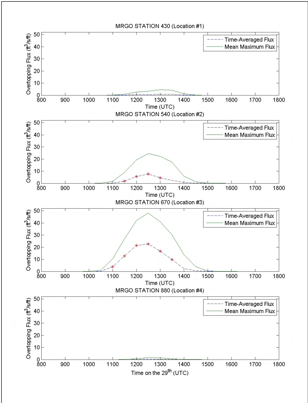
Figure 171. Overtopping rates for all four locations shown in Figure 164
