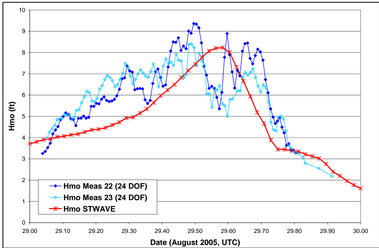
Figure 55. Lake Pontchartrain measured and modeled significant wave height
