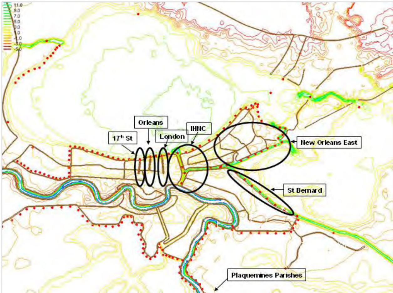
Figure 140. Geographic area analyzed within scope of detailed hydrodynamics portion of report
