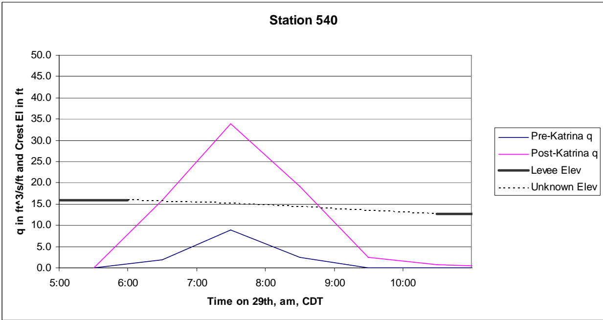
Figure 176. Approximate overtopping rate and levee crest height during storm as a function of time for Station 540 using Equation 1
