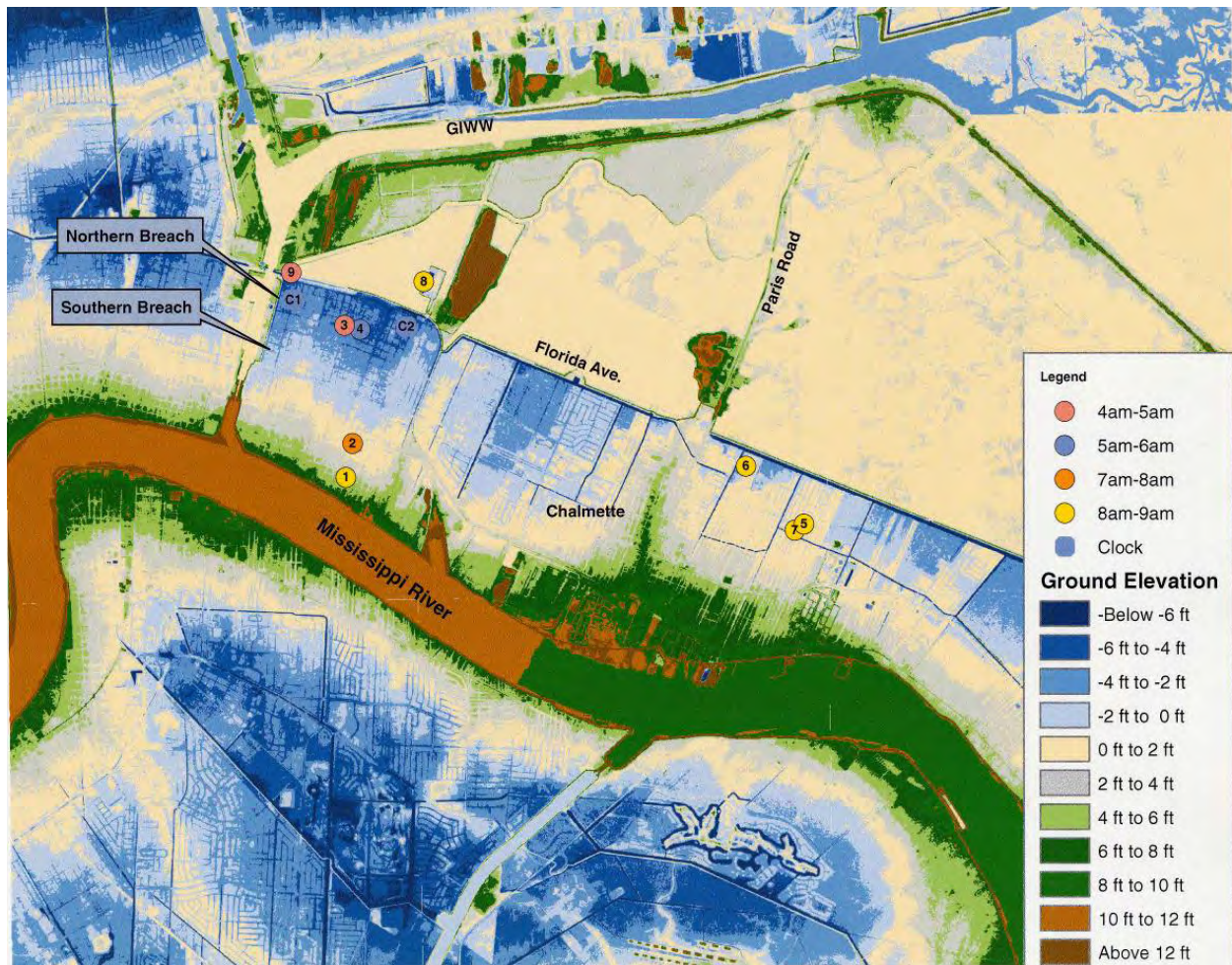
Figure 135. Lower Ninth Ward and St Bernard Parish study area with locations of eyewitness accounts and stopped clocks
