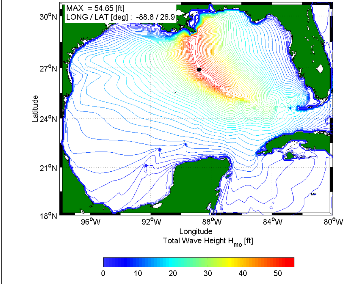
Figure 37. Color contour of the maximum wave height conditions in the Basin domain
