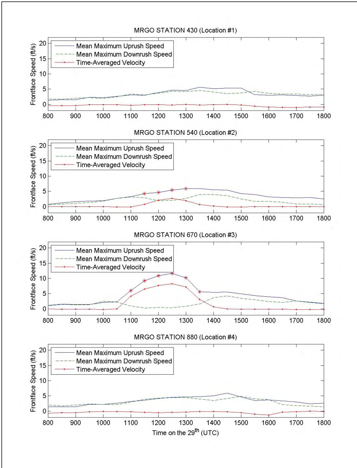
Figure 169. Velocities along the front face of the levees at the four locations shown in Figure 164
