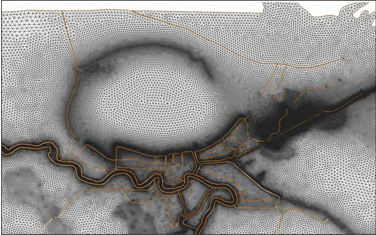
Figure 73. Bathymetry/topography used in the ADCIRC storm surge model (TF01x2 grid); Lake Pontchartrain vicinity
