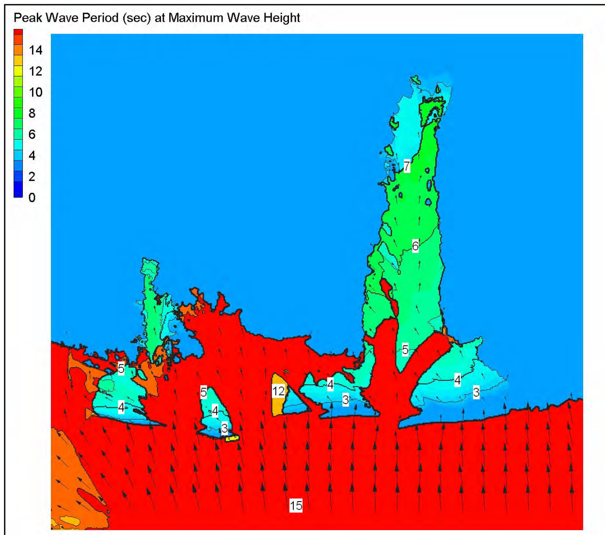
Figure 67. Mississippi-Alabama modeled peak wave period and corresponding mean wave direction (periods in sec)
