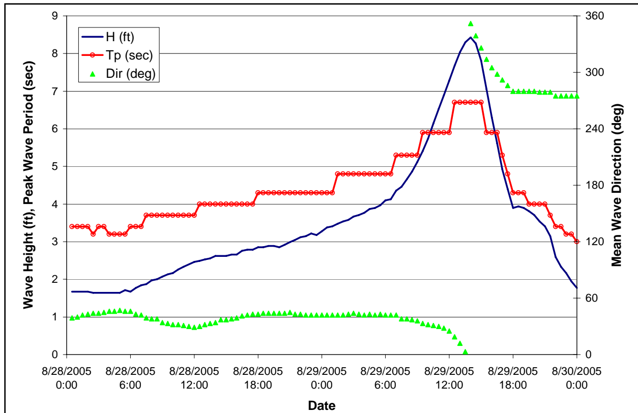
Figure 54. Temporal variation of significant wave height, peak period, and mean wave direction along the south shore of Lake Pontchartrain
