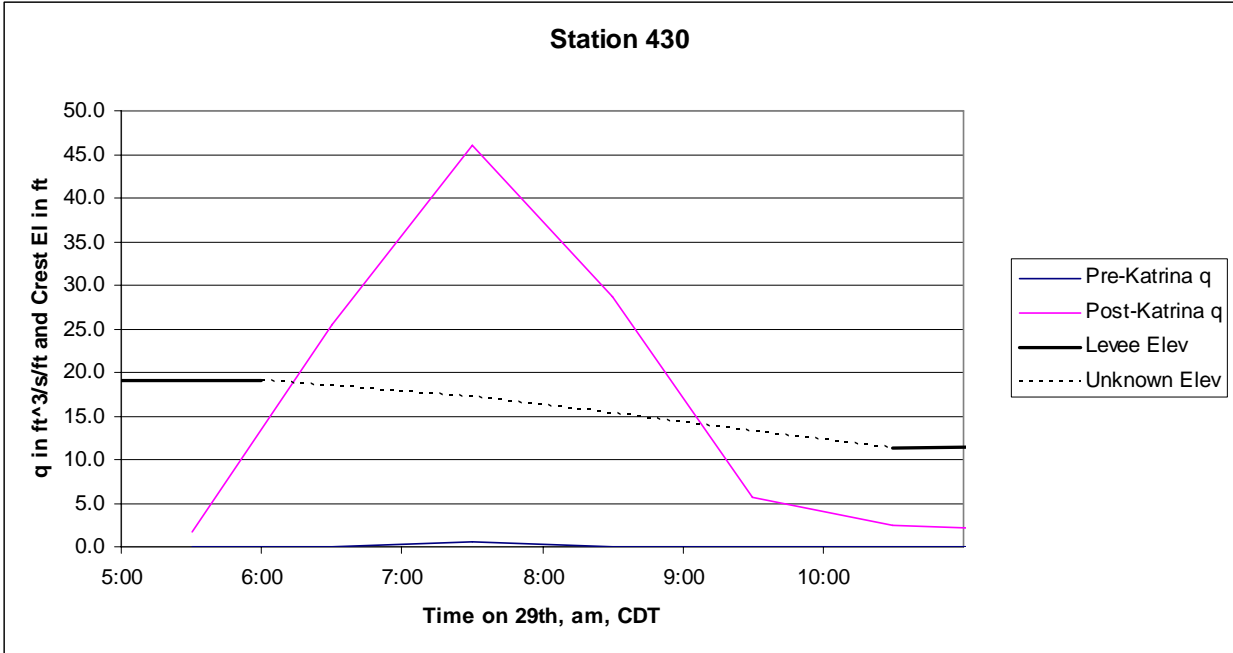
Figure 175. Approximate overtopping rate and levee crest height during storm as a function of time for Station 430 using Equation 1
