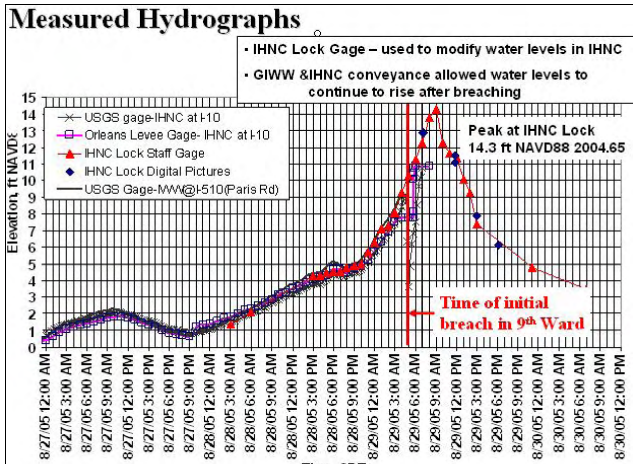
Figure 159. Hydrograph of water levels measured at gages within the IHNC. Vertical line designates approximate time of initial flooding in Lower Ninth Ward
