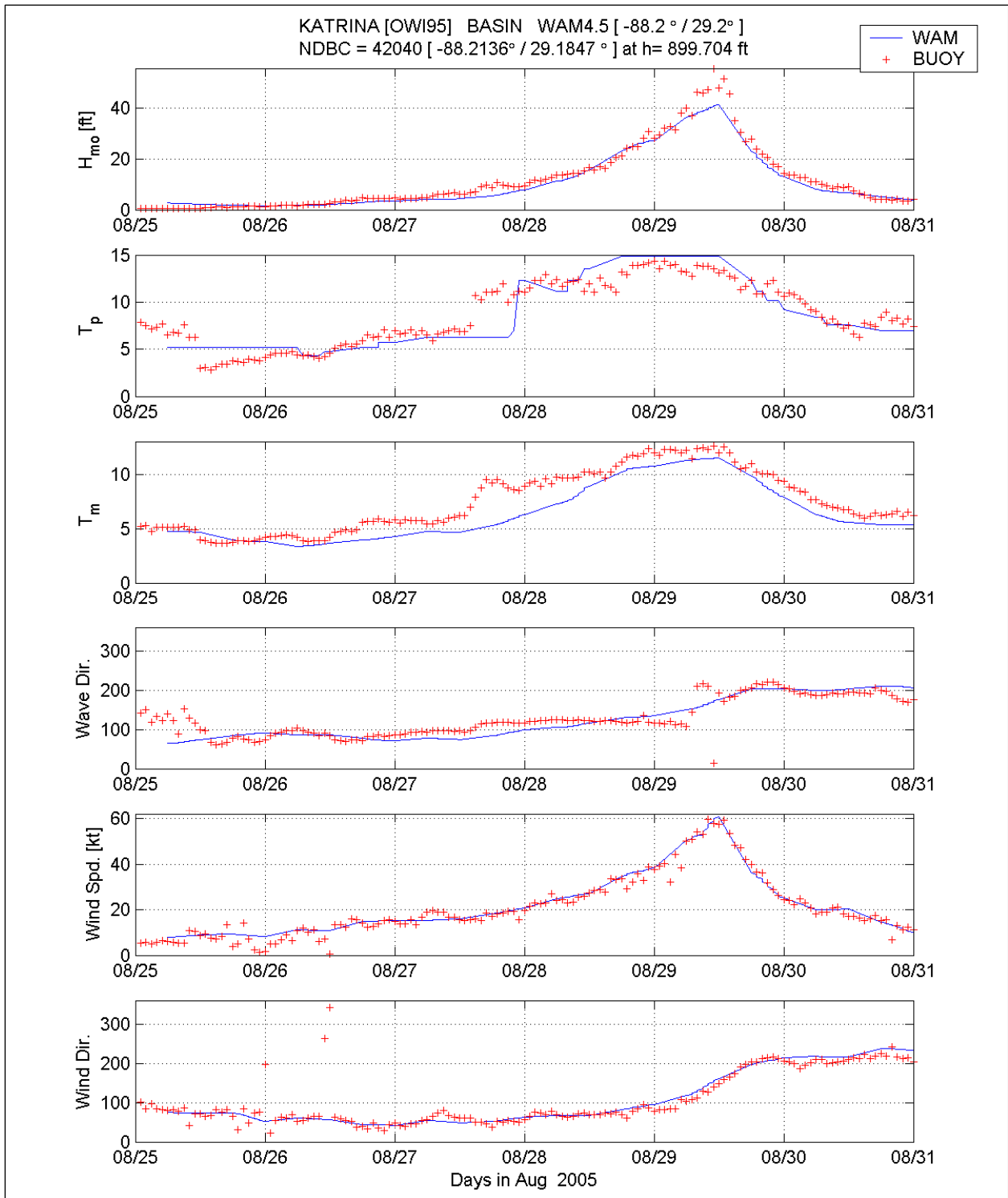
Figure 40. Comparison of WAM Cycle 4.5 basin-scale (blue line) to the measurements at NDBC 42040
