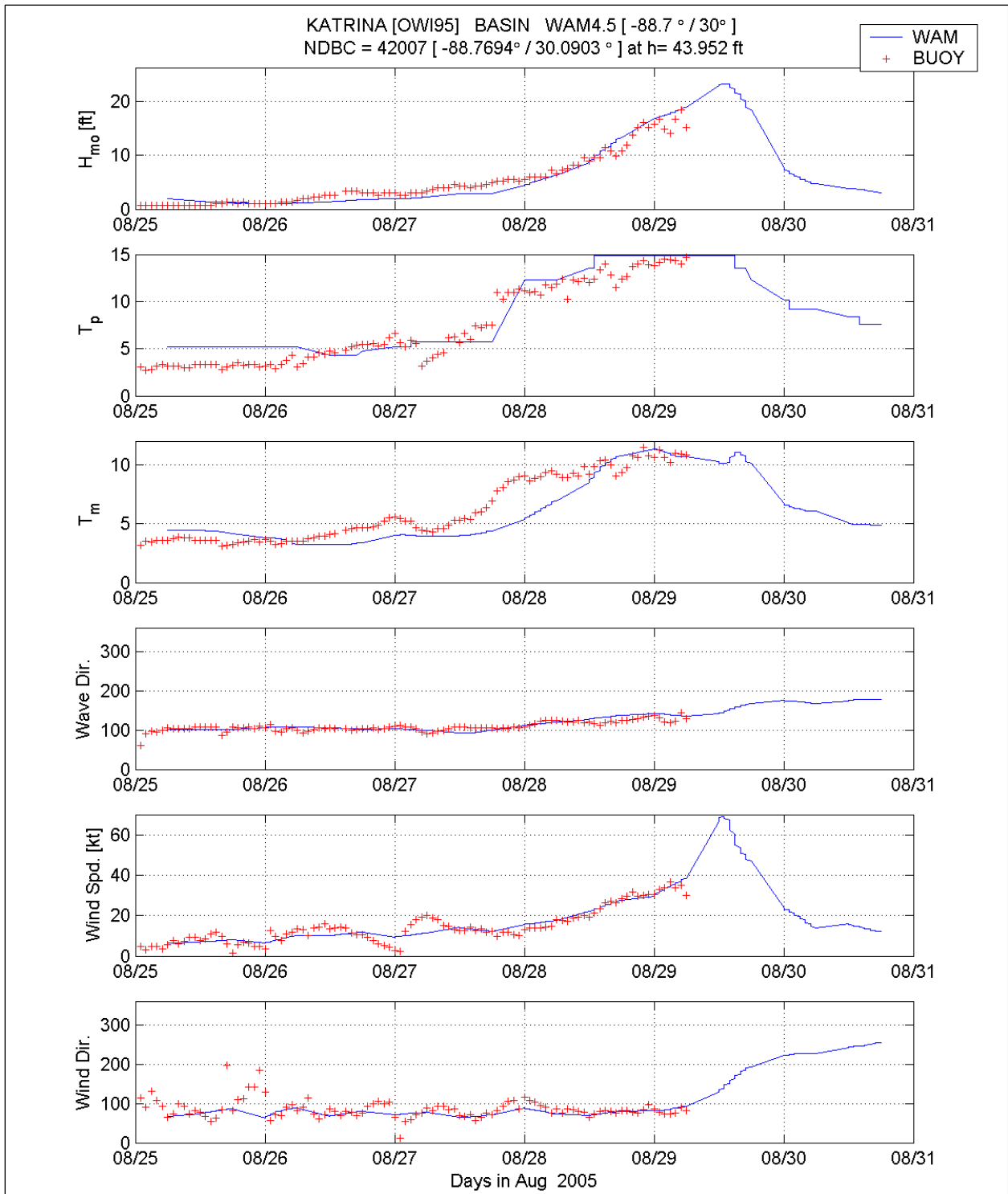
Figure 41. Comparison of WAM Cycle 4.5 basin-scale (blue line) to the measurements at NDBC 42007
