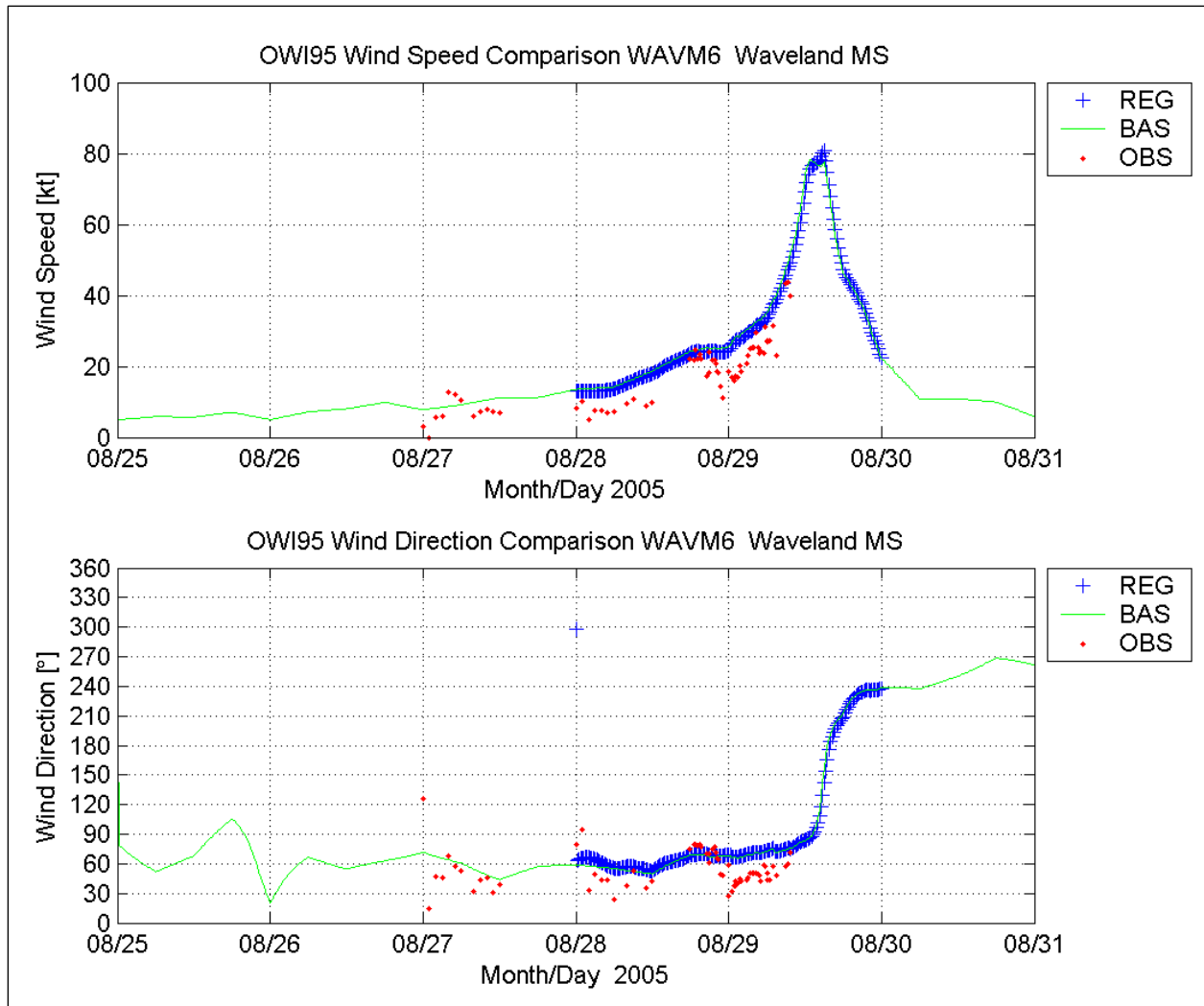
Figure 31. Comparison of wind speed (upper panel) and direction (bottom panel) at Waveland, MS
