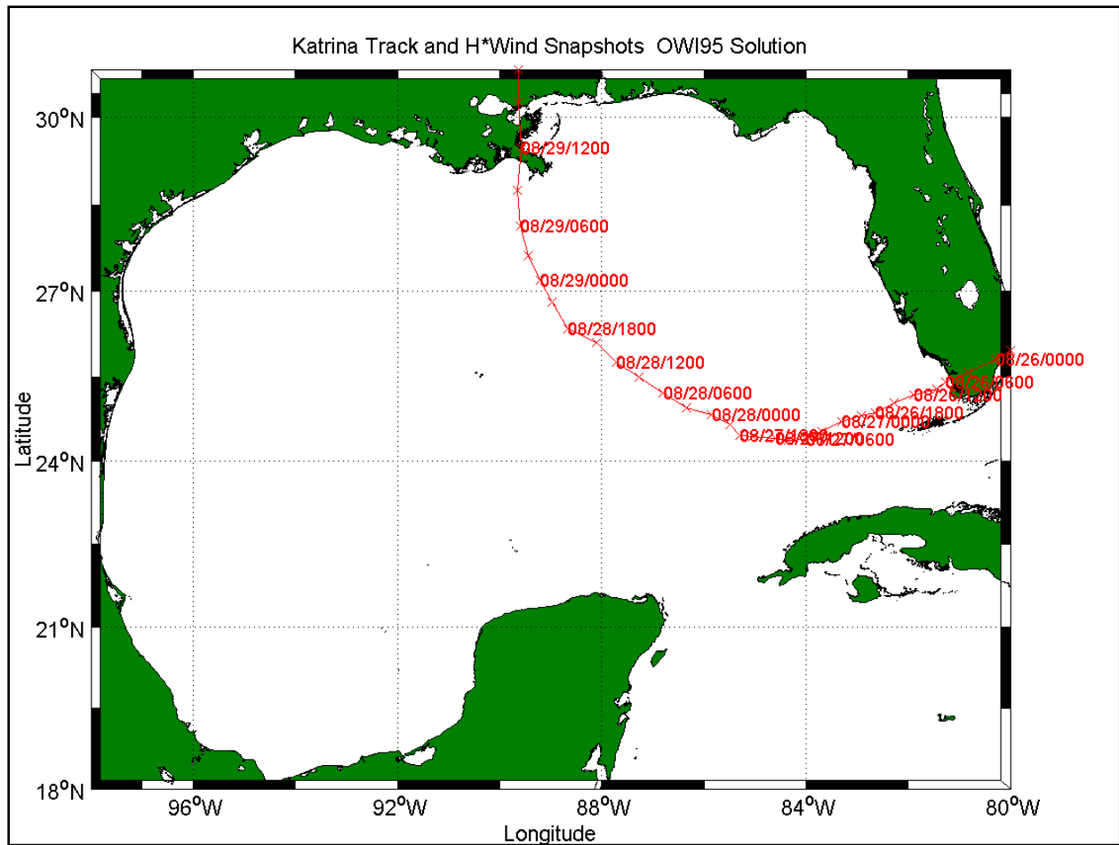
Figure 1. Hurricane Katrina track and times of H*wind snapshots
