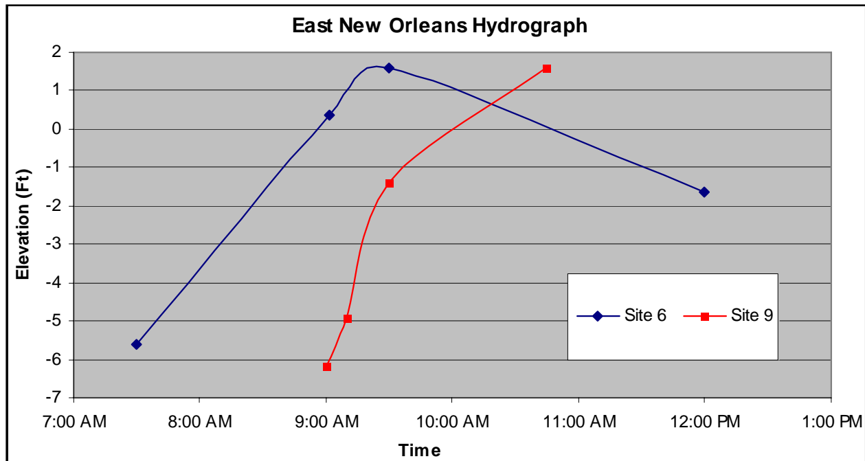
Figure 134. New Orleans East hydrographs based on surveyed elevations of eyewitness accounts at sites 6 and 9.
