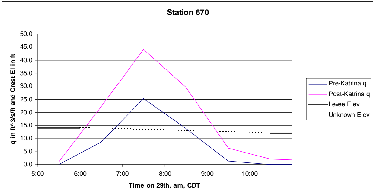
Figure 177. Approximate overtopping rate and levee crest height during storm as a function of time for Station 670 using Equation 1
