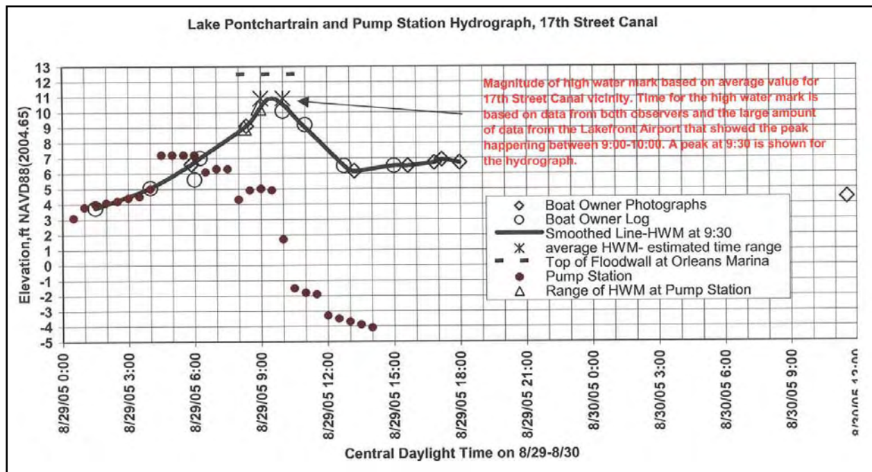
Figure 144. Estimated water levels in Lake Pontchartrain near north end of 17th Street Canal. The solid line is used for analysis purposes here
