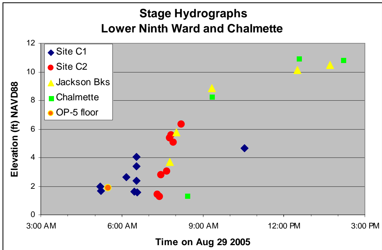
Figure 136. Chalmette and Lower Ninth Ward hydrographs
