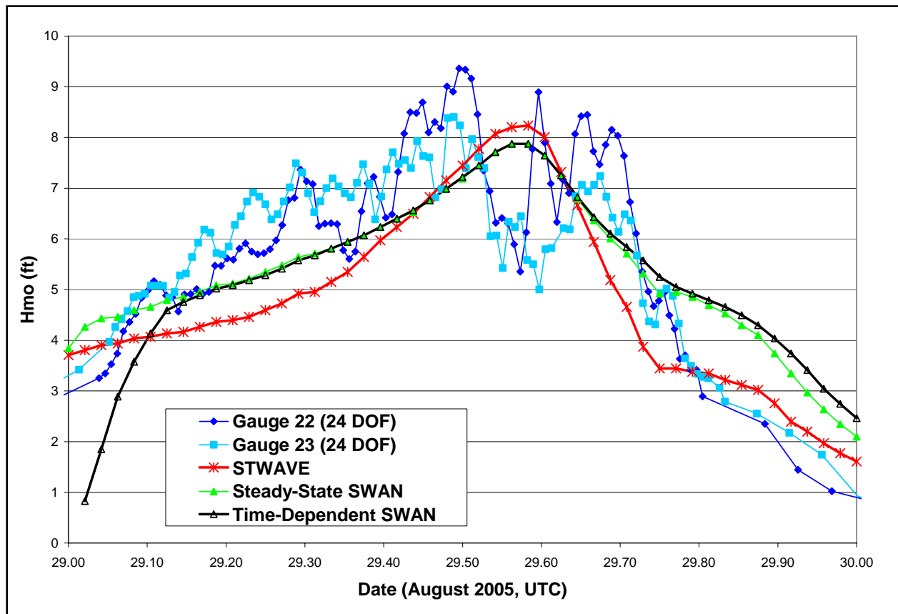
Figure 68. Time-dependent and steady-state SWAN and STWAVE modeled significant wave heights for Lake Pontchartrain and measured significant wave height
