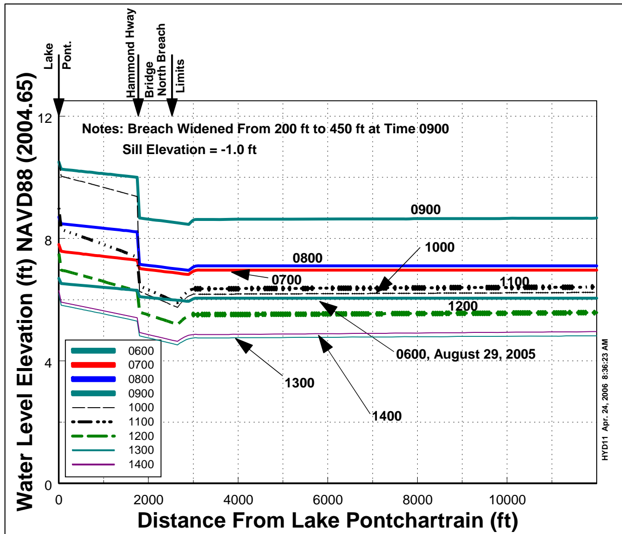
Figure 150. Water levels along 17th Street Canal. Scenario 1
