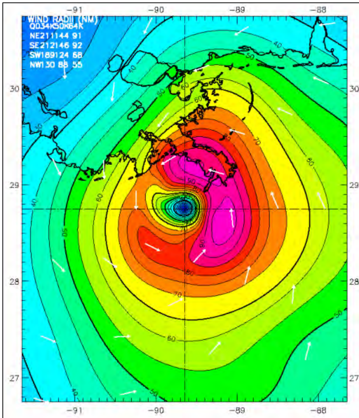
Figure 25. H*Wind snapshot for 0900 UTC on August 29, just prior to landfall
