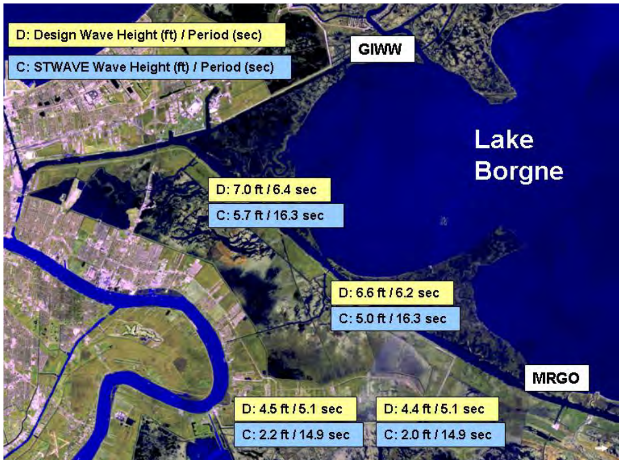
Figure 86. Wave maxima along hurricane protection system of St. Bernard Parish
