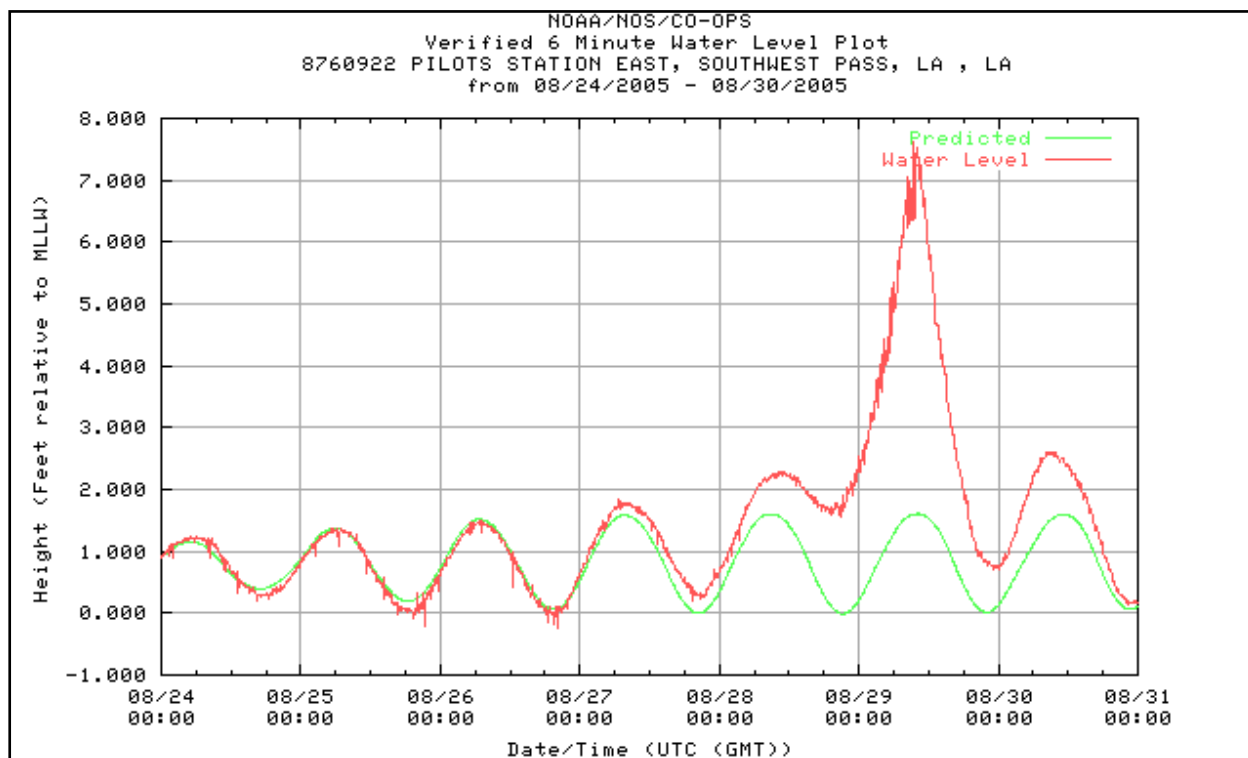
Figure 24. Hydrograph for NOAA National Ocean Service Station at Southwest Pass, Louisiana
