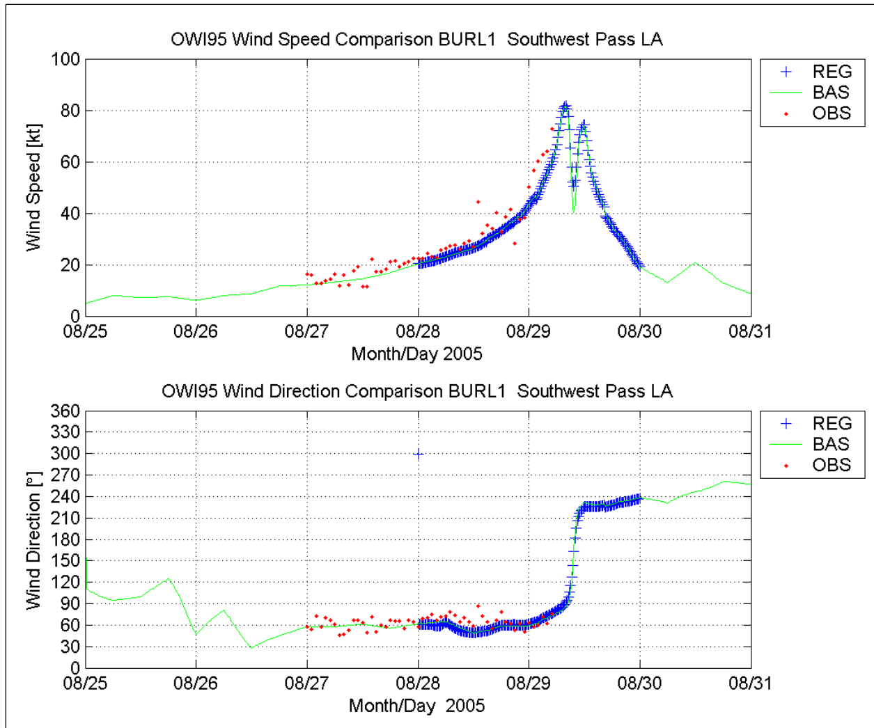
Figure 29. Comparison of wind speed (upper panel) and direction (bottom panel) at Southwest Pass, LA
