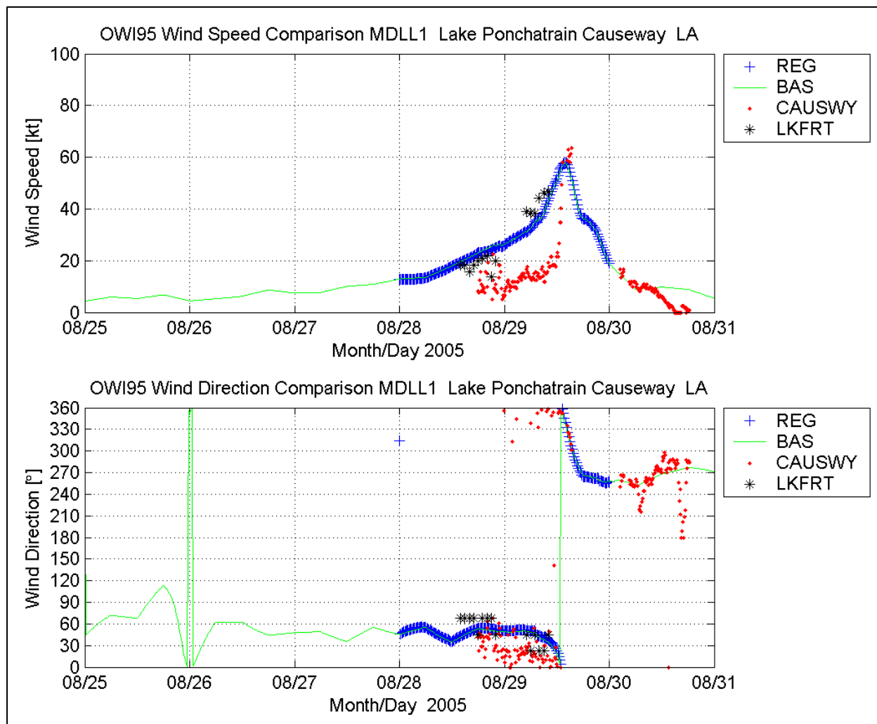
Figure 32. Comparison of wind speed (upper panel) and direction (bottom panel) at Mid Lake, Lake Pontchartrain, LA
