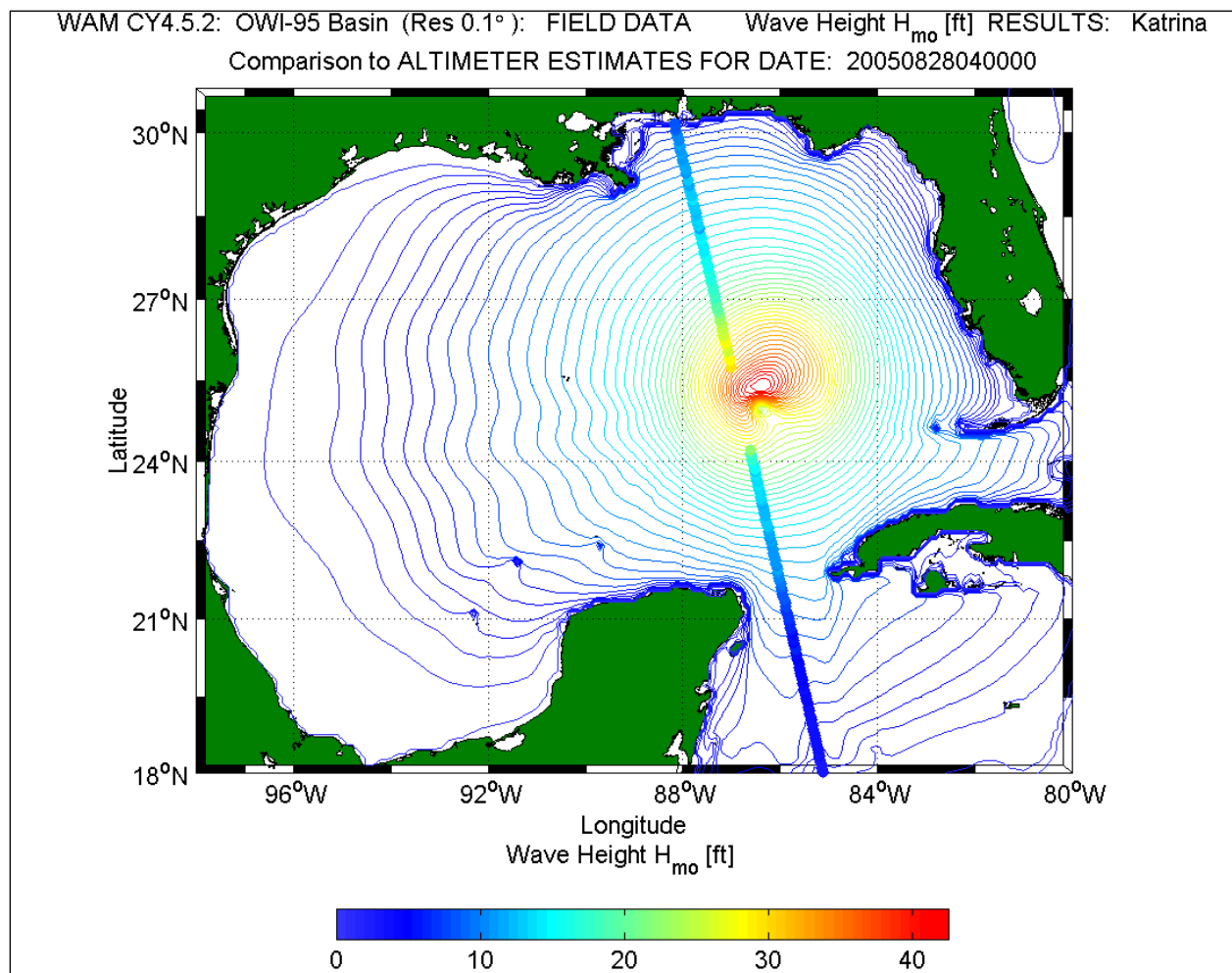
Figure 42. WAM wave height color contour overlaying ENVSAT altimeter wave height estimates at 28 August 2005 0400 UTC.
