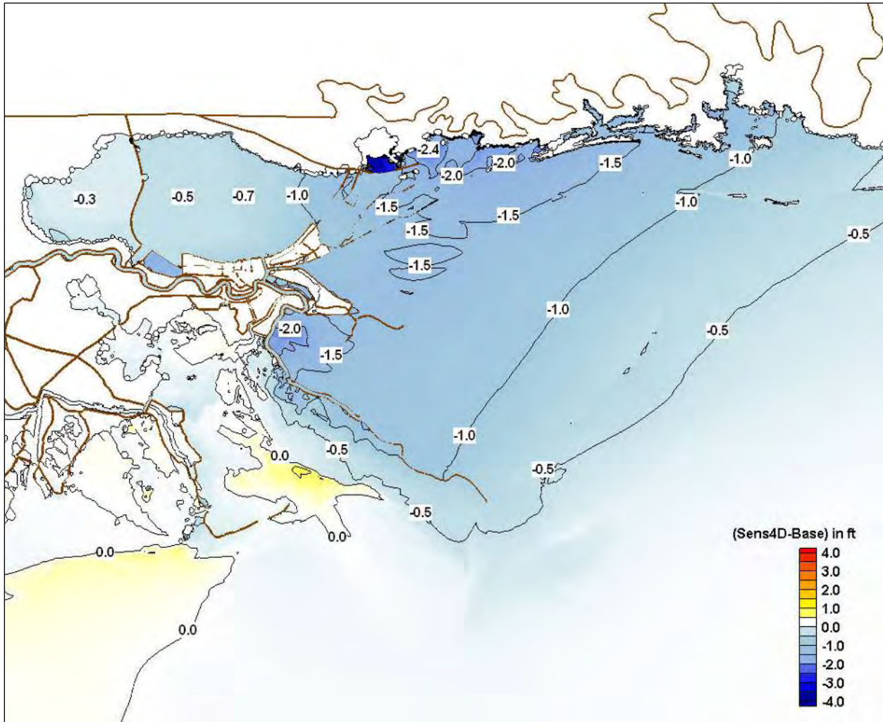
Figure 97. Difference in peak surge between sensitivity simulation with 5% decrease in wind speed and the base simulation
