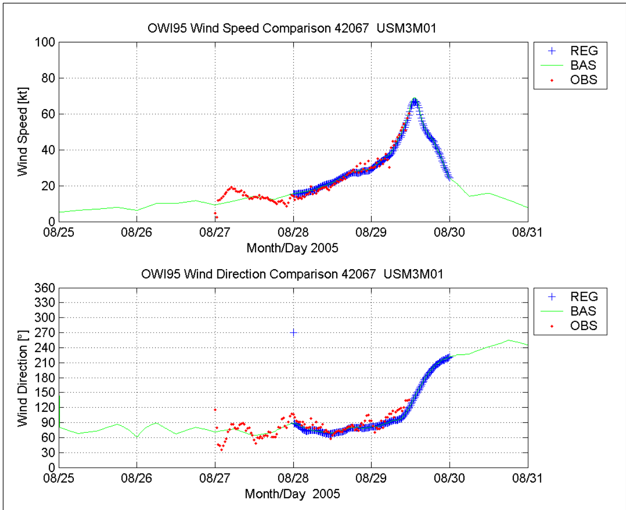
Figure 30. Comparison of wind speed (upper panel) and direction (bottom panel) at Buoy 42067
