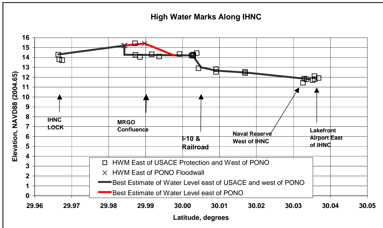
Figure 18. Variation of peak water level along IHNC based on high water marks
