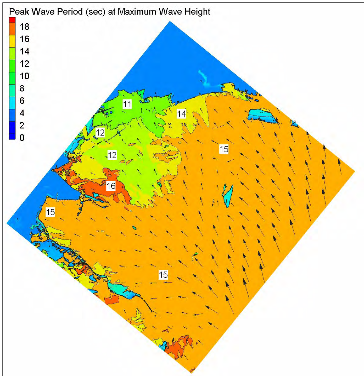
Figure 59. Southeast Louisiana modeled peak wave period corresponding to the maximum significant wave height (periods in sec)
