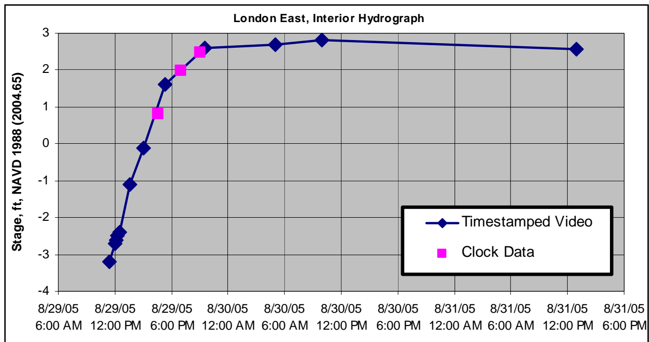
Figure 125. Stage hydrograph for London East based on video at site 34
