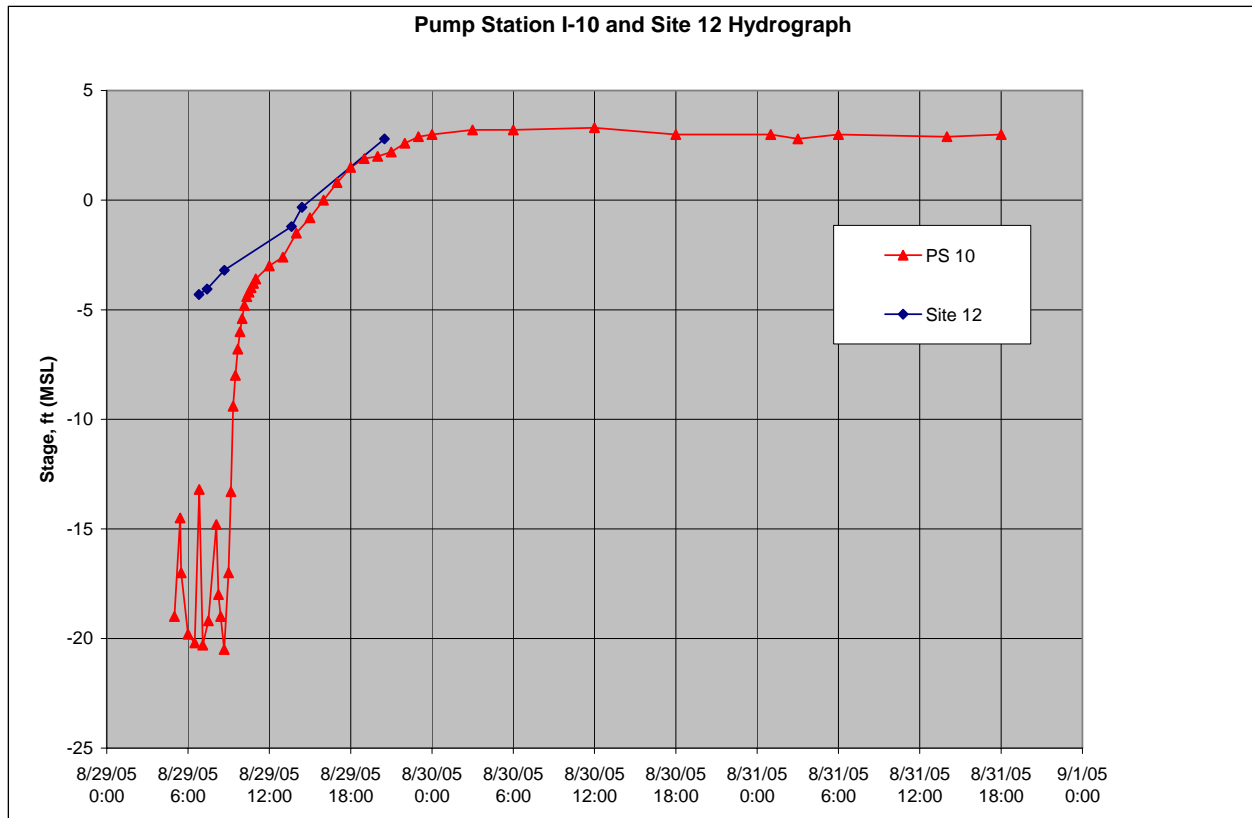
Figure 117. Stage hydrograph at Pump Station 10 and at Site 12.
