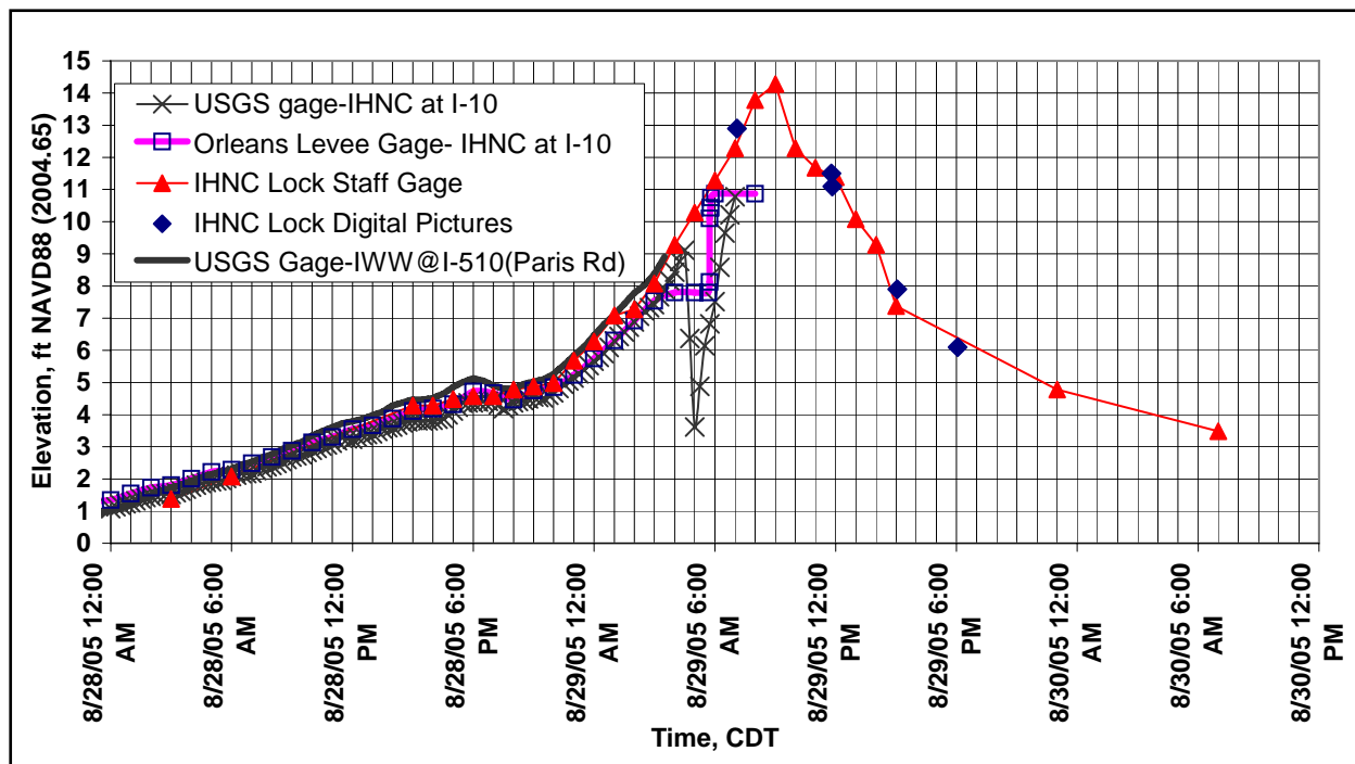
Figure 14. Hydrographs on the IHNC and GIWW
